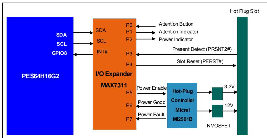
Figure 1 Hot-Plug via I/O Expander Block Diagram
