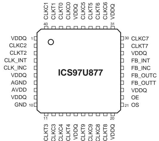
40-Pin MLF
