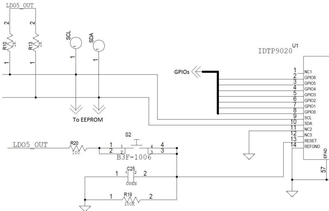
Figure 8d. Detail of RESET and I2C connections.
