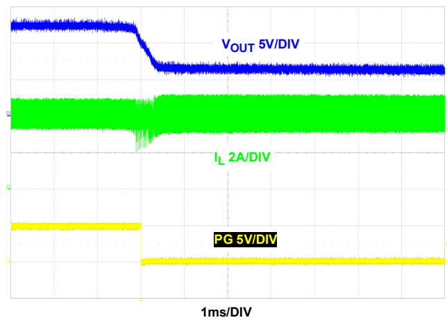
FIGURE 36. OVERCURRENT PROTECTION
