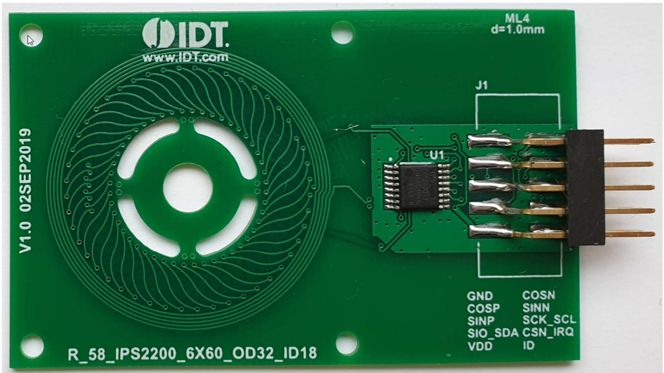
Figure 1. Sensor Board
