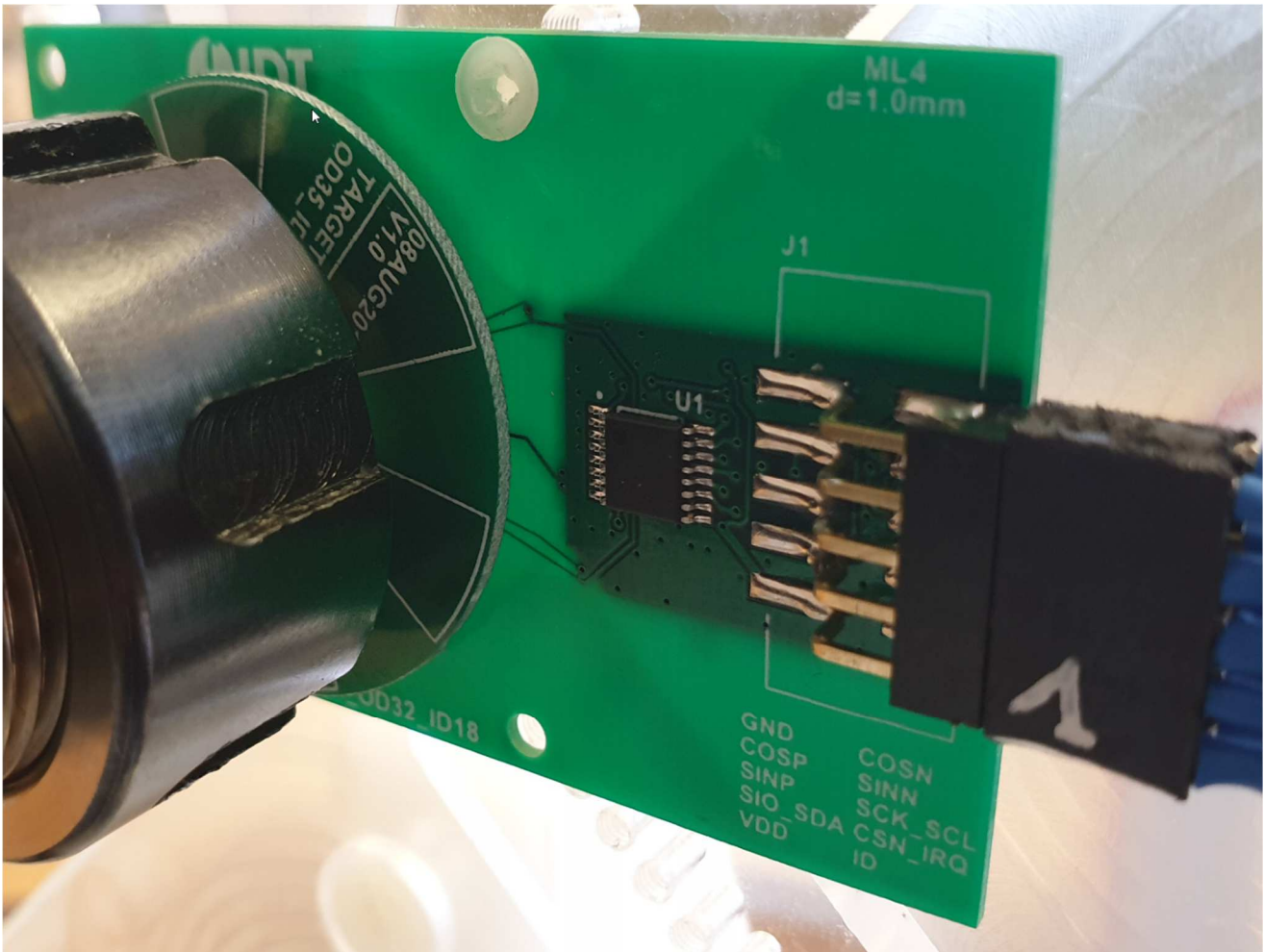
Figure 3. Setup
