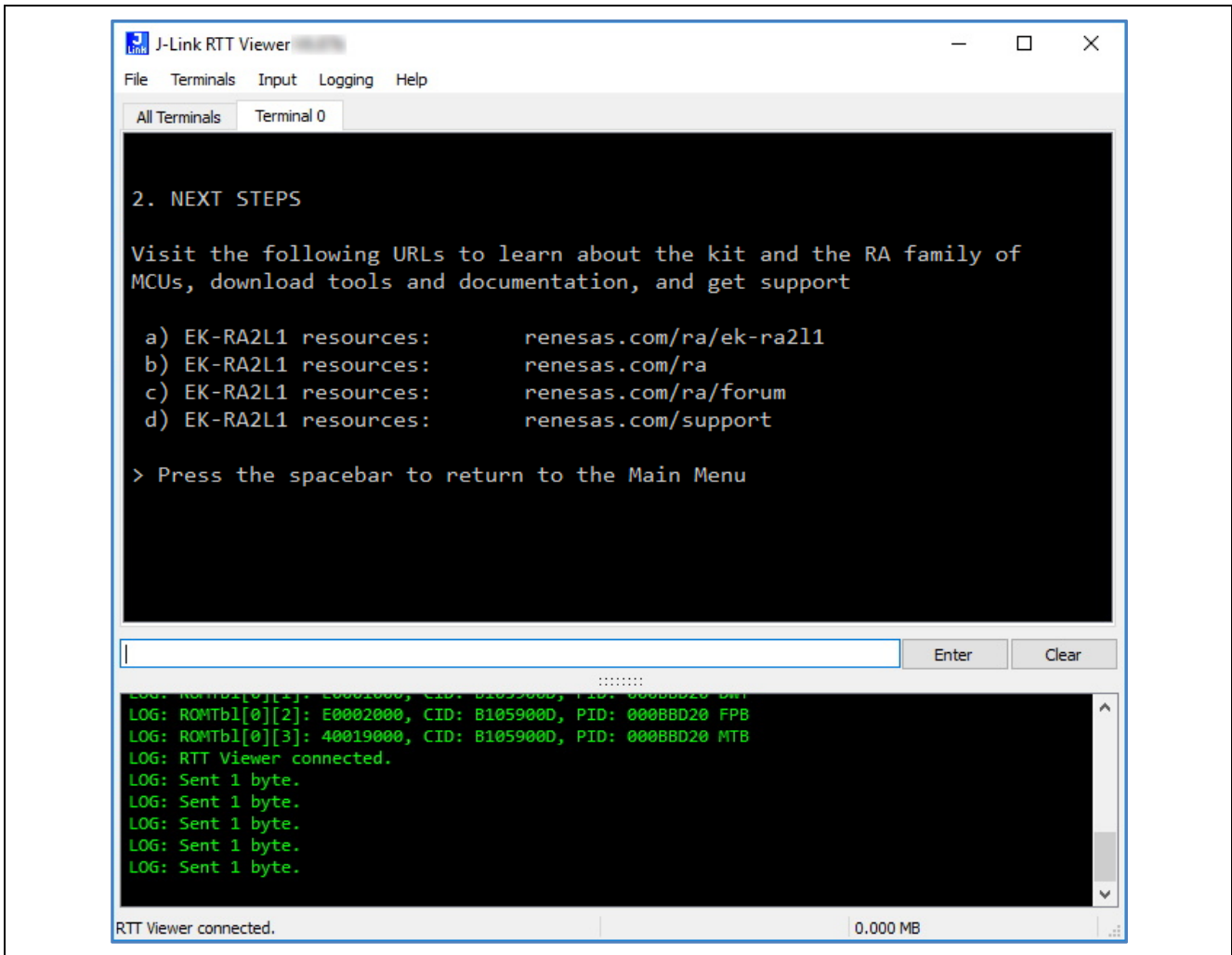
Figure 8. Next Steps
