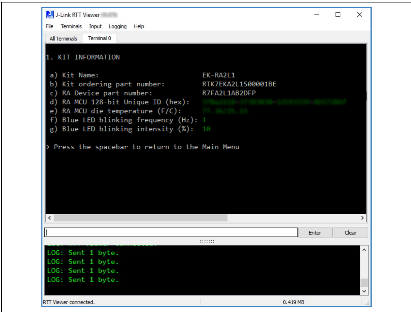
Figure 7. Kit Information
