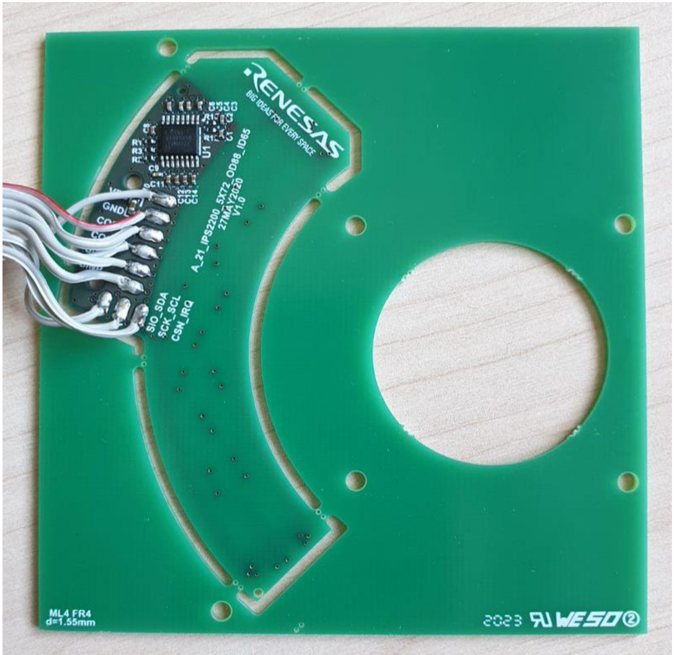
Figure 1. Sensor Board
