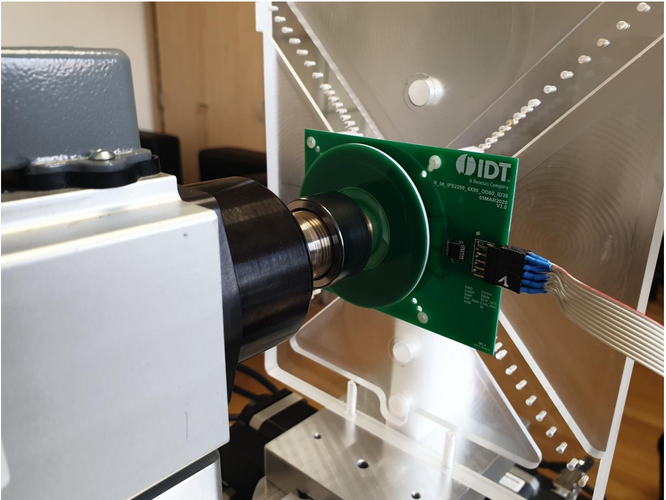
Figure 3. Setup
