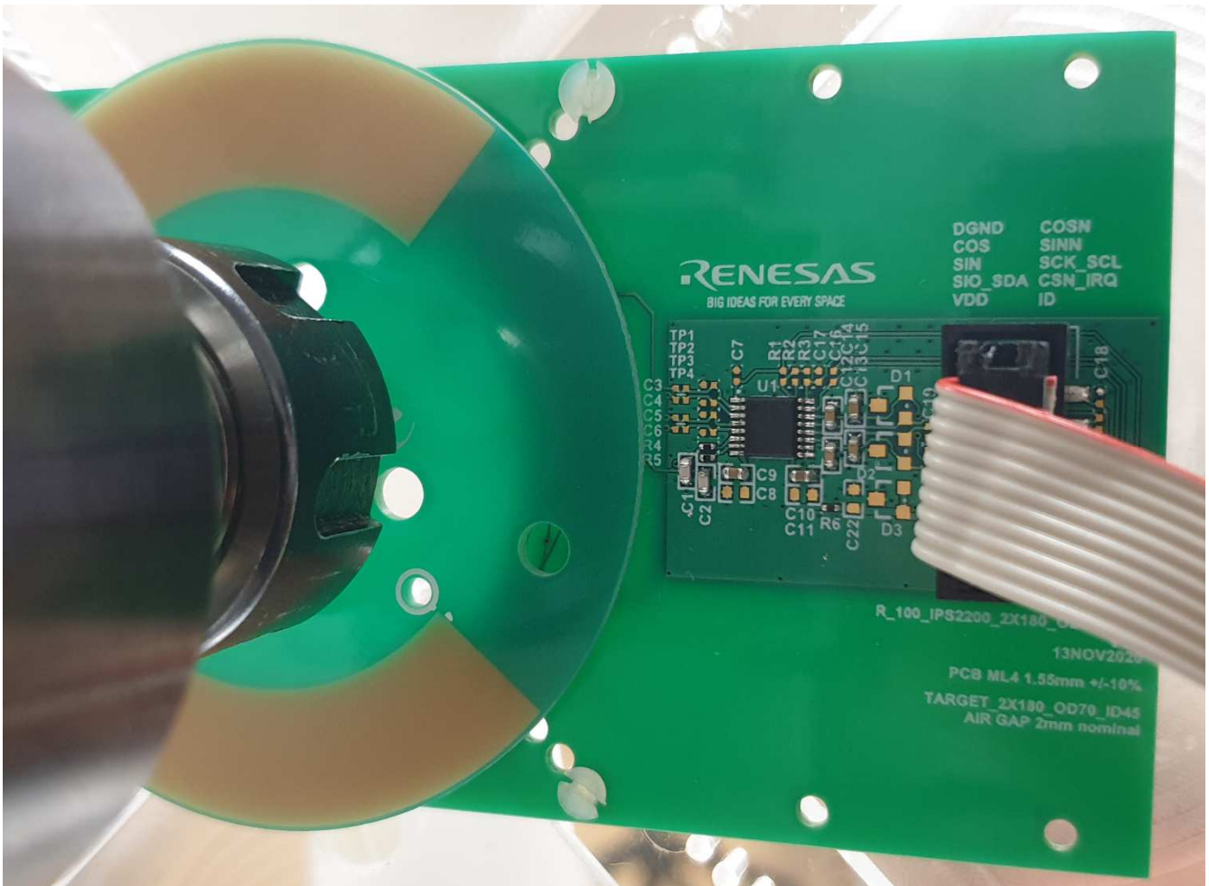
Figure 3. Setup
