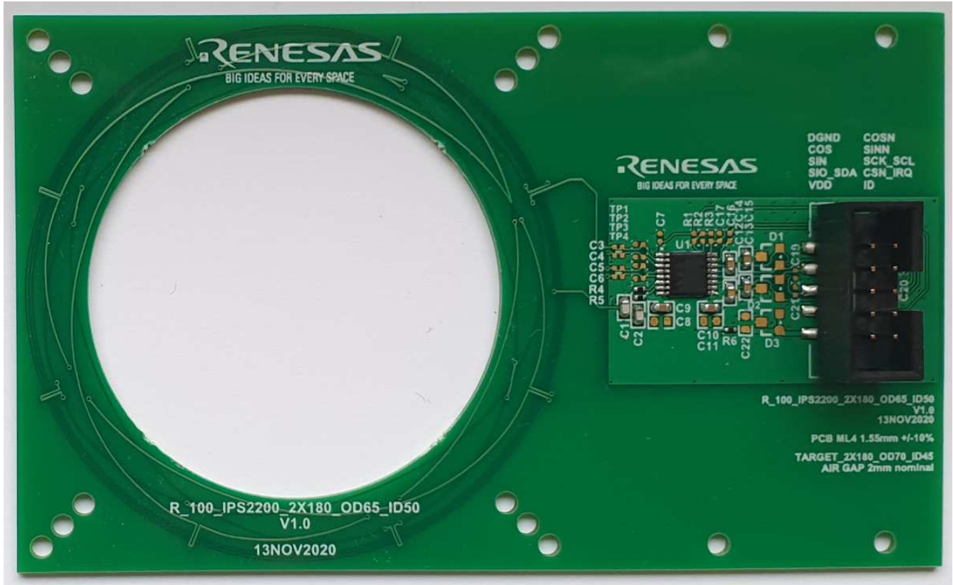
Figure 1. Sensor Board
