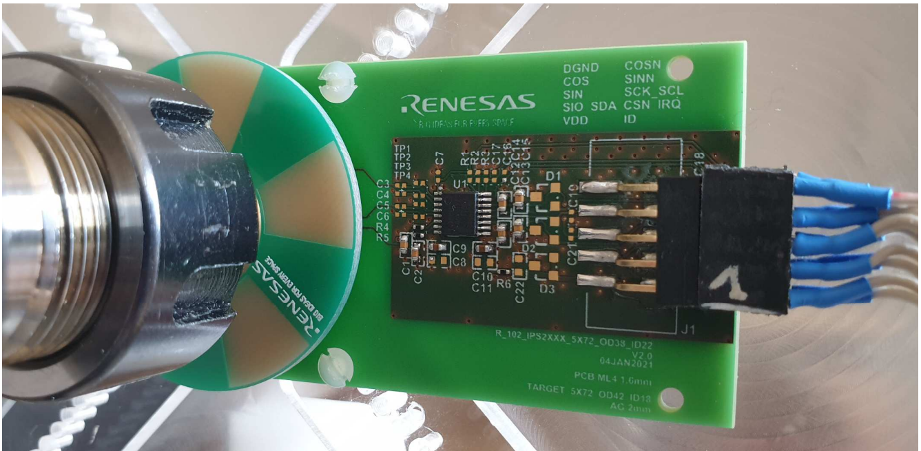
Figure 3. Setup
