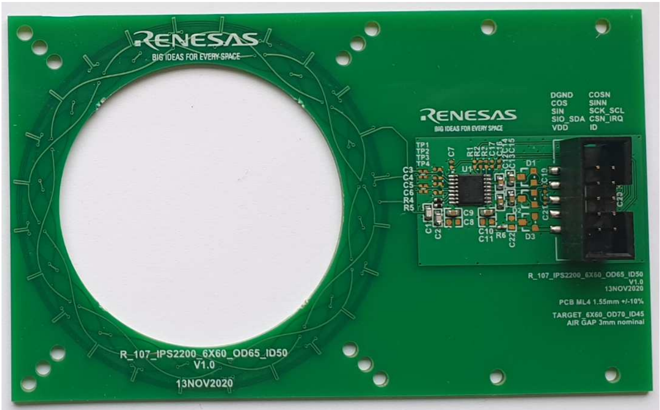
Figure 1. Sensor Board
