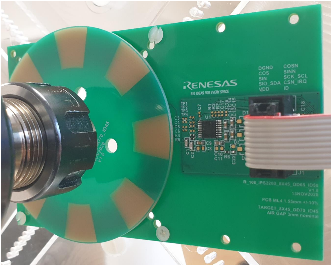
Figure 3. Setup
