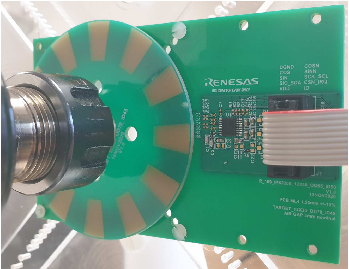
Figure 3. Setup
