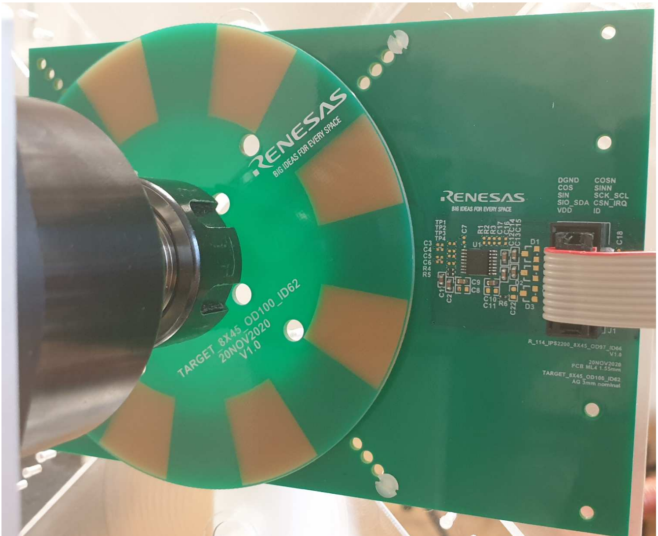
Figure 3. Setup
