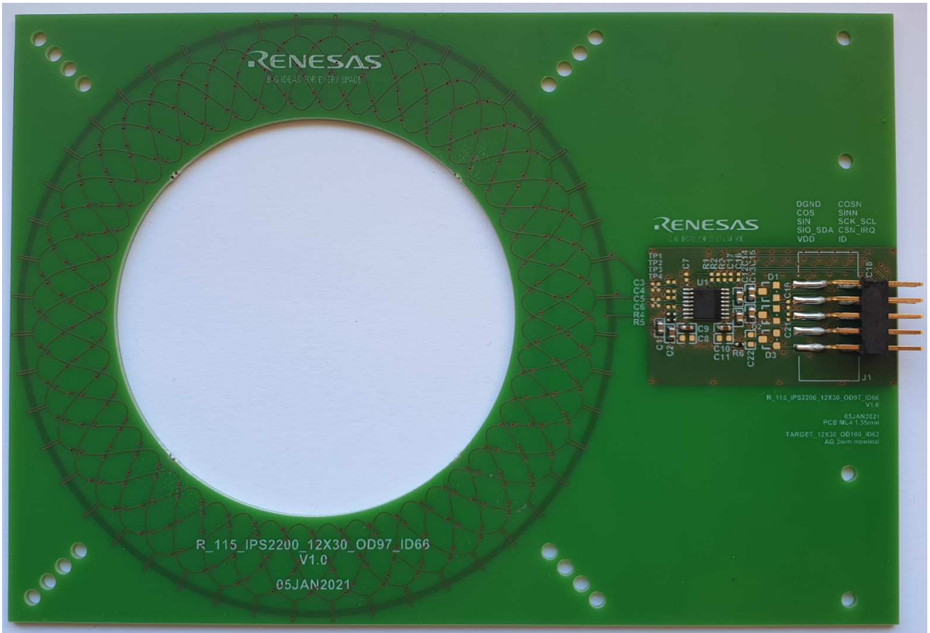
Figure 1. Sensor Board
