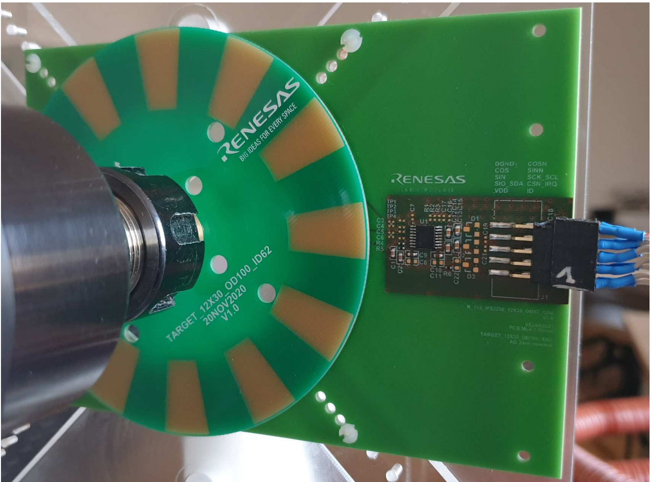
Figure 3. Setup
