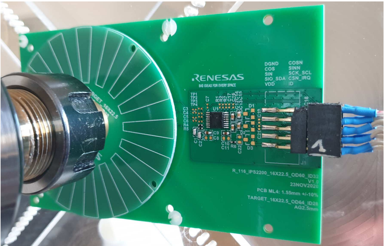
Figure 3. Setup
