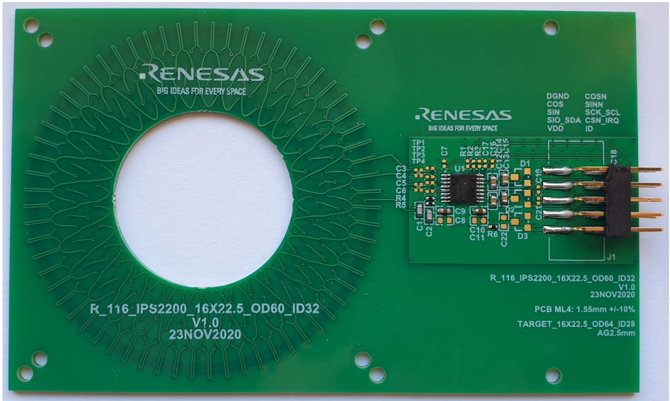
Figure 1. Sensor Board
