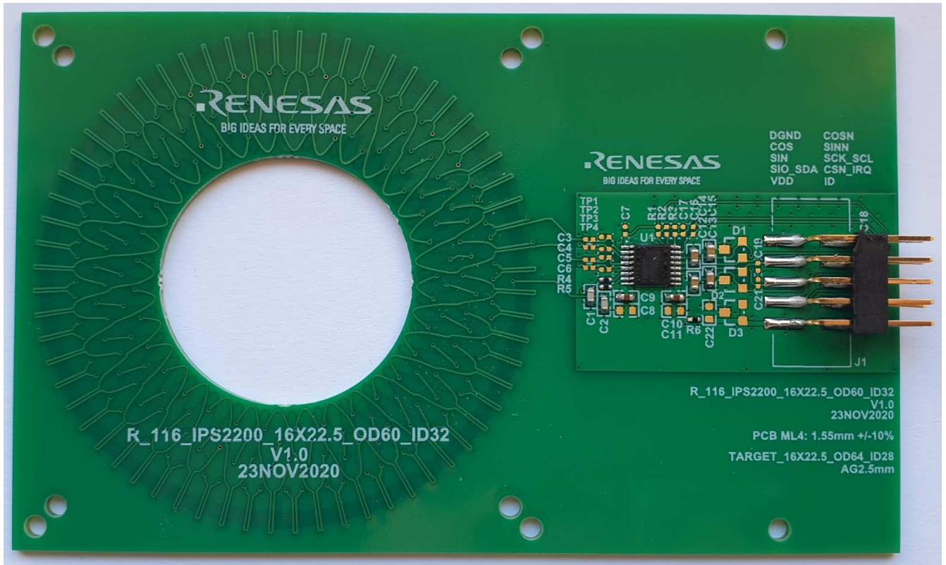
Figure 1. Sensor Board
