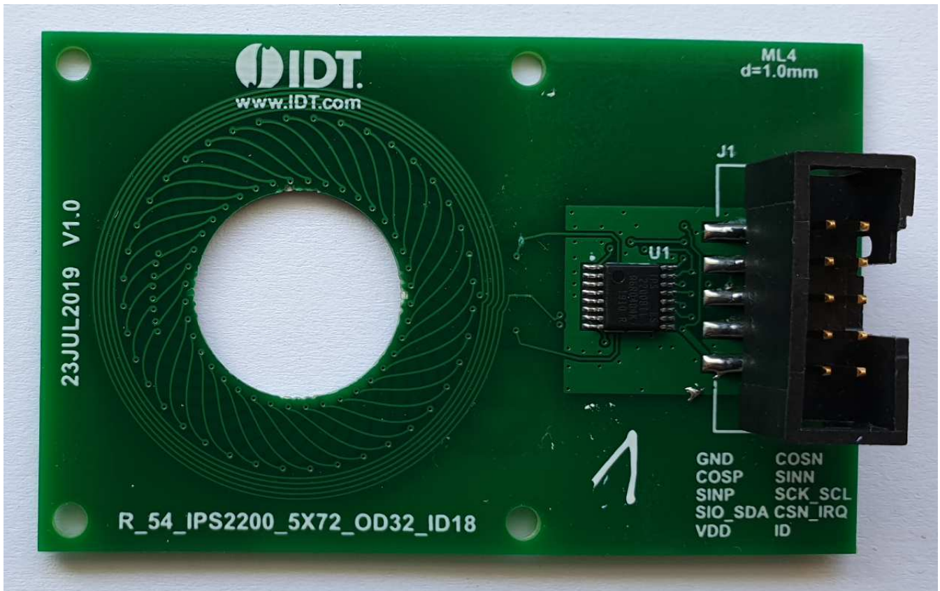
Figure 1. Sensor Board
