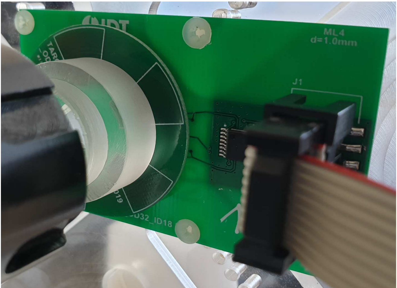
Figure 3. Setup
