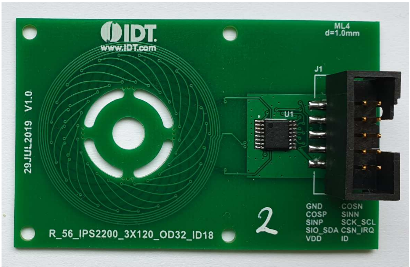
Figure 1. Sensor Board
