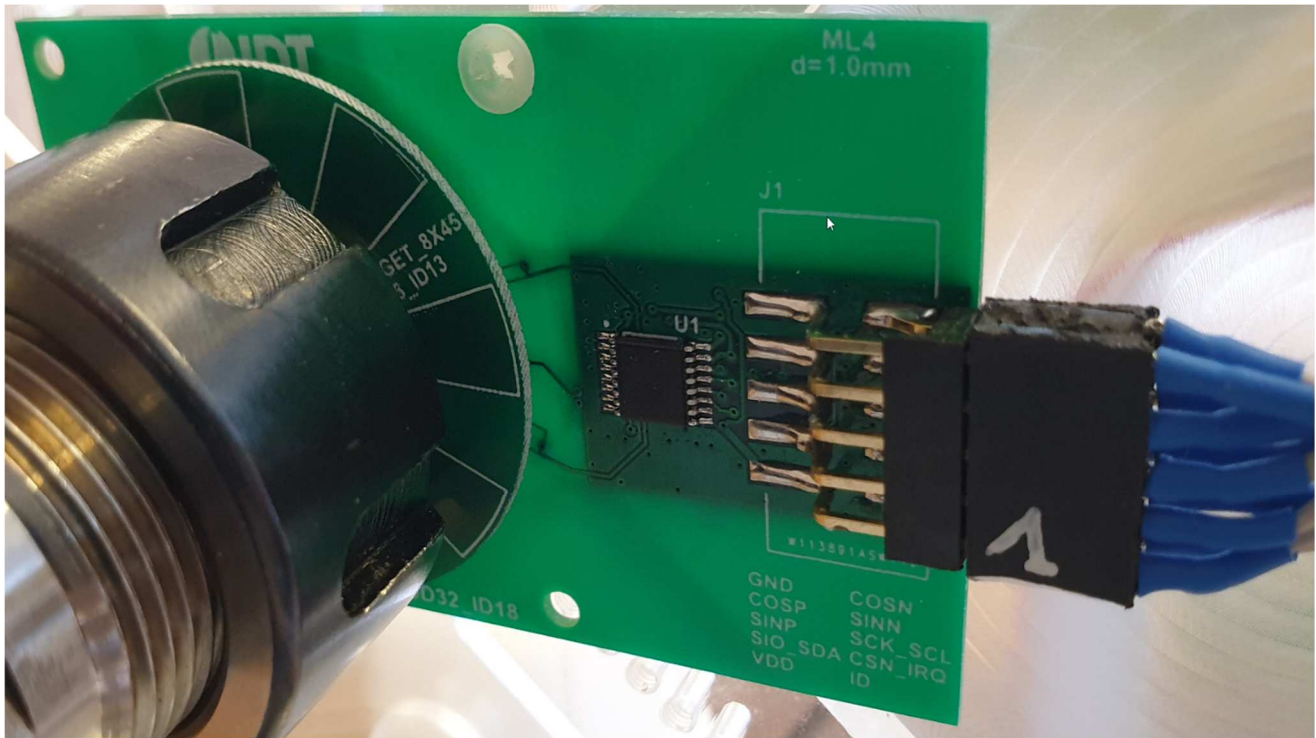
Figure 3. Setup
