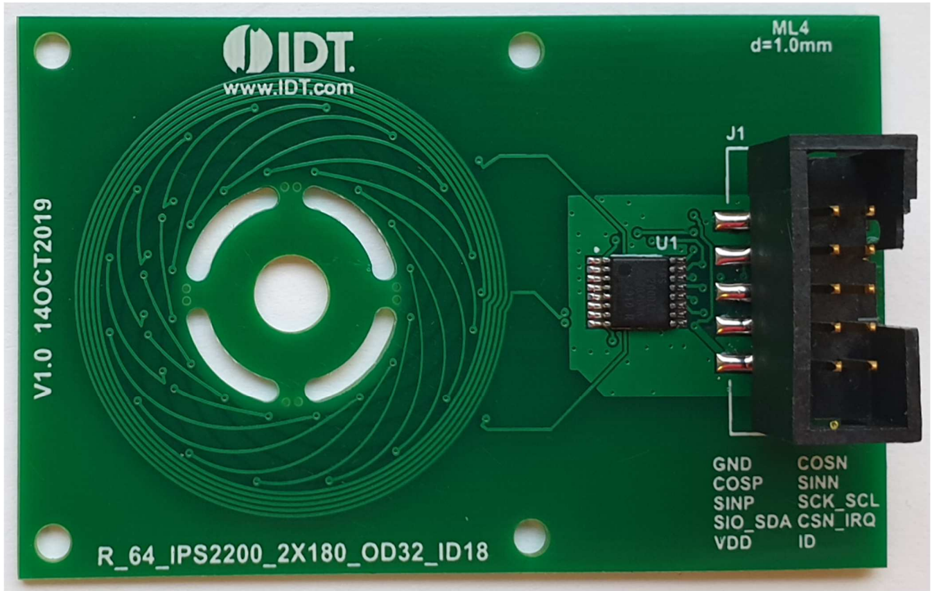
Figure 1. Sensor Board
