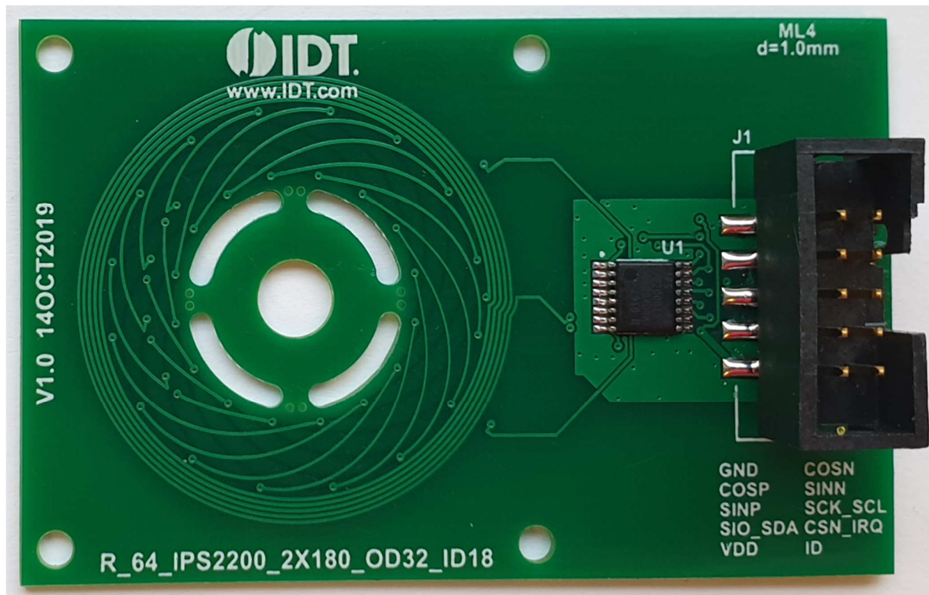
Figure 1. Sensor Board
