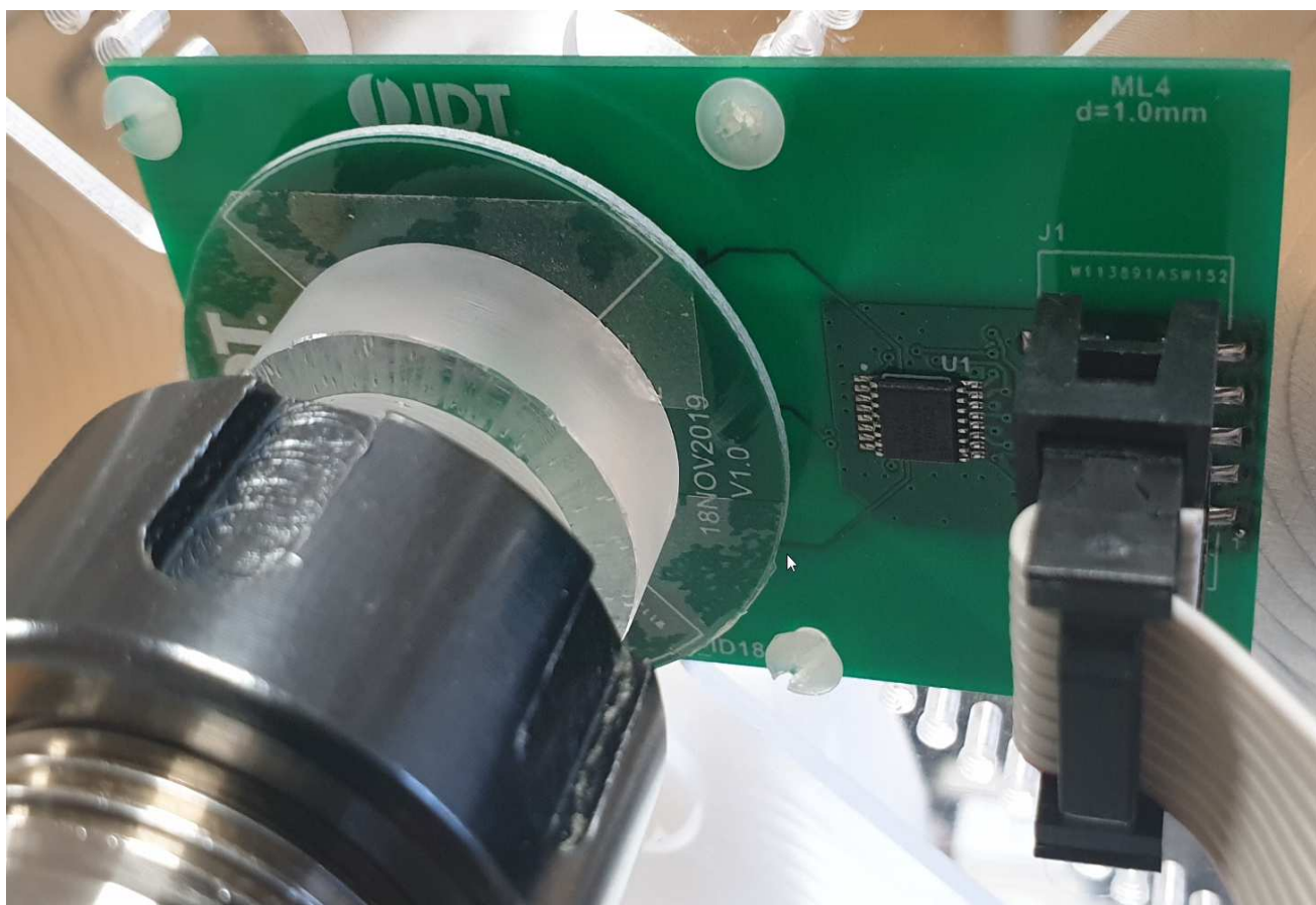
Figure 3. Setup
