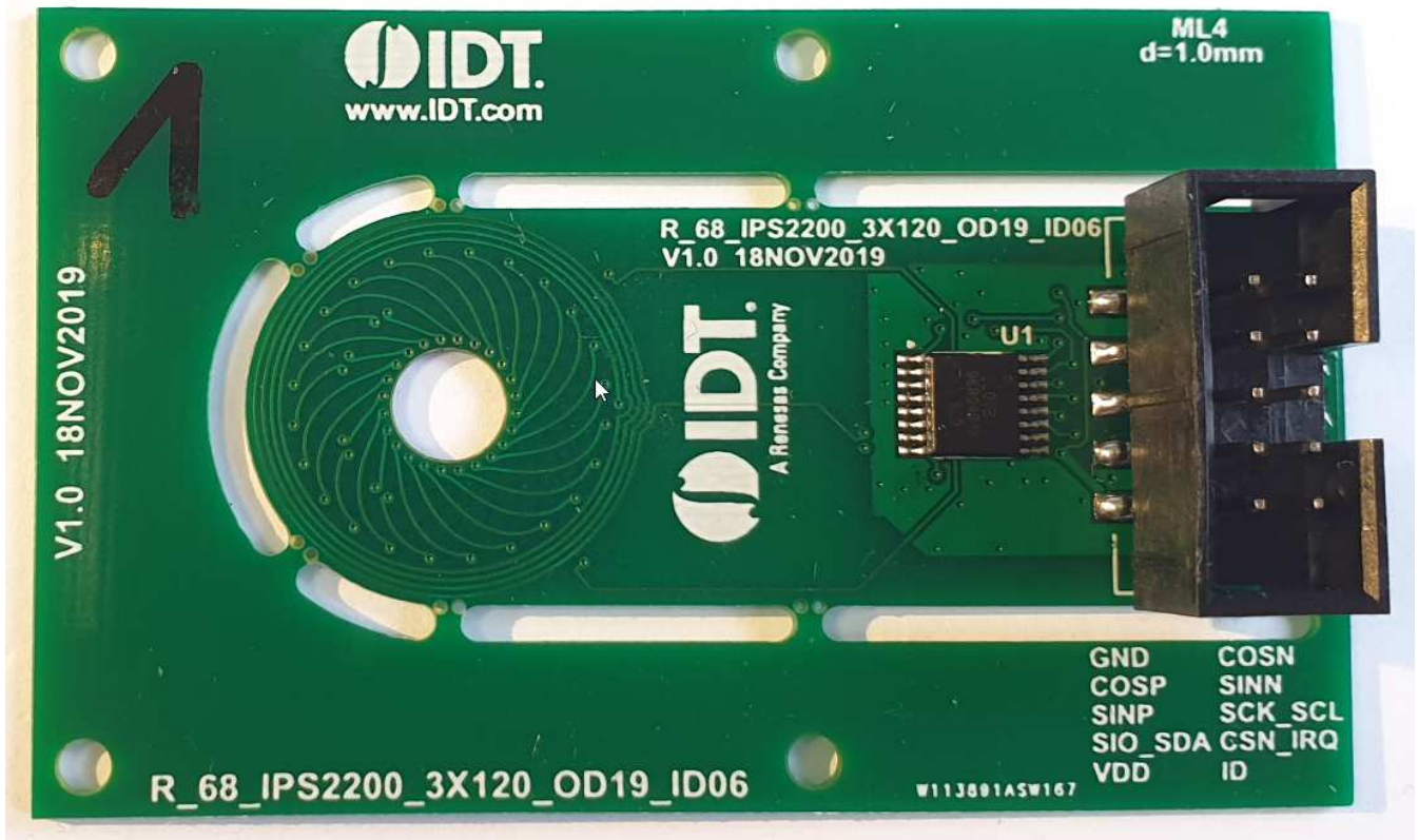
Figure 1. Sensor Board
