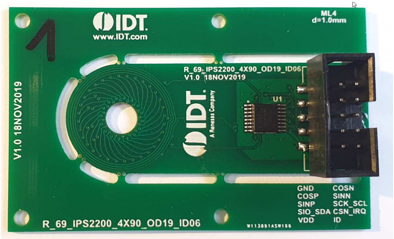
Figure 1. Sensor Board
