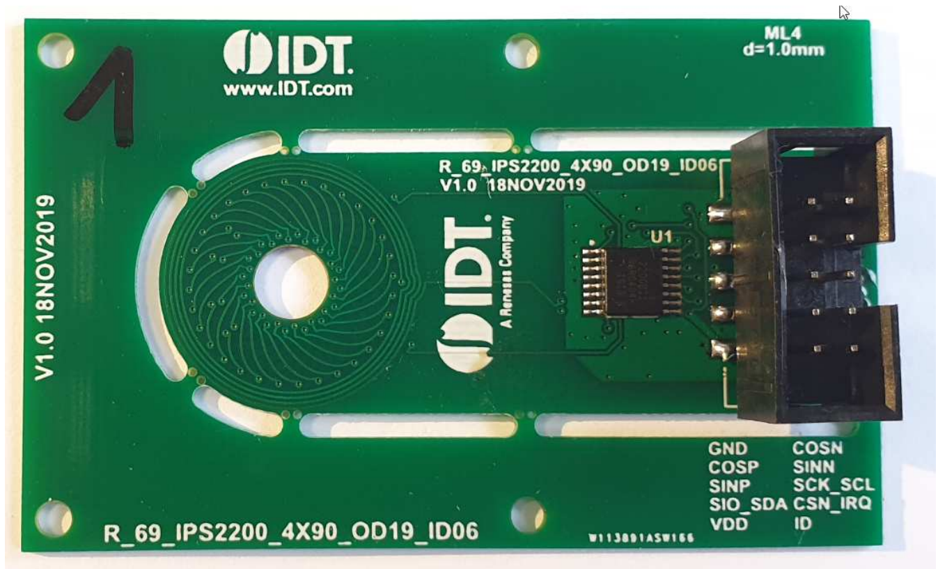
Figure 1. Sensor Board
