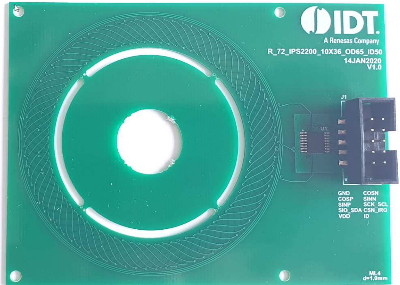
Figure 1. Sensor Board
