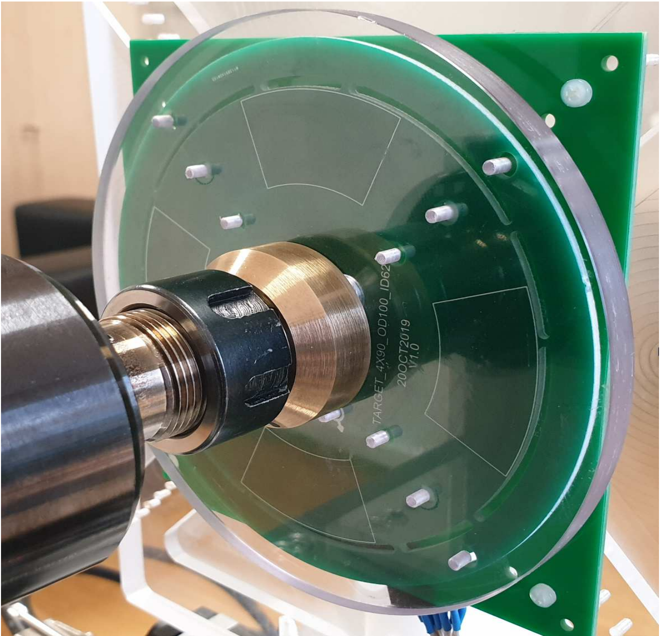
Figure 3. Setup
