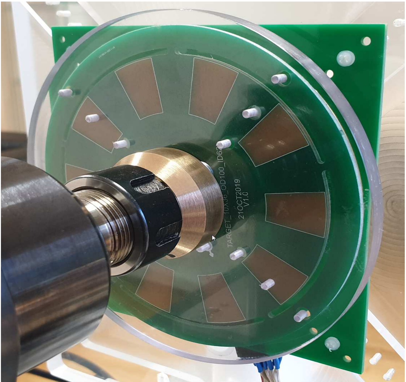
Figure 3. Setup
