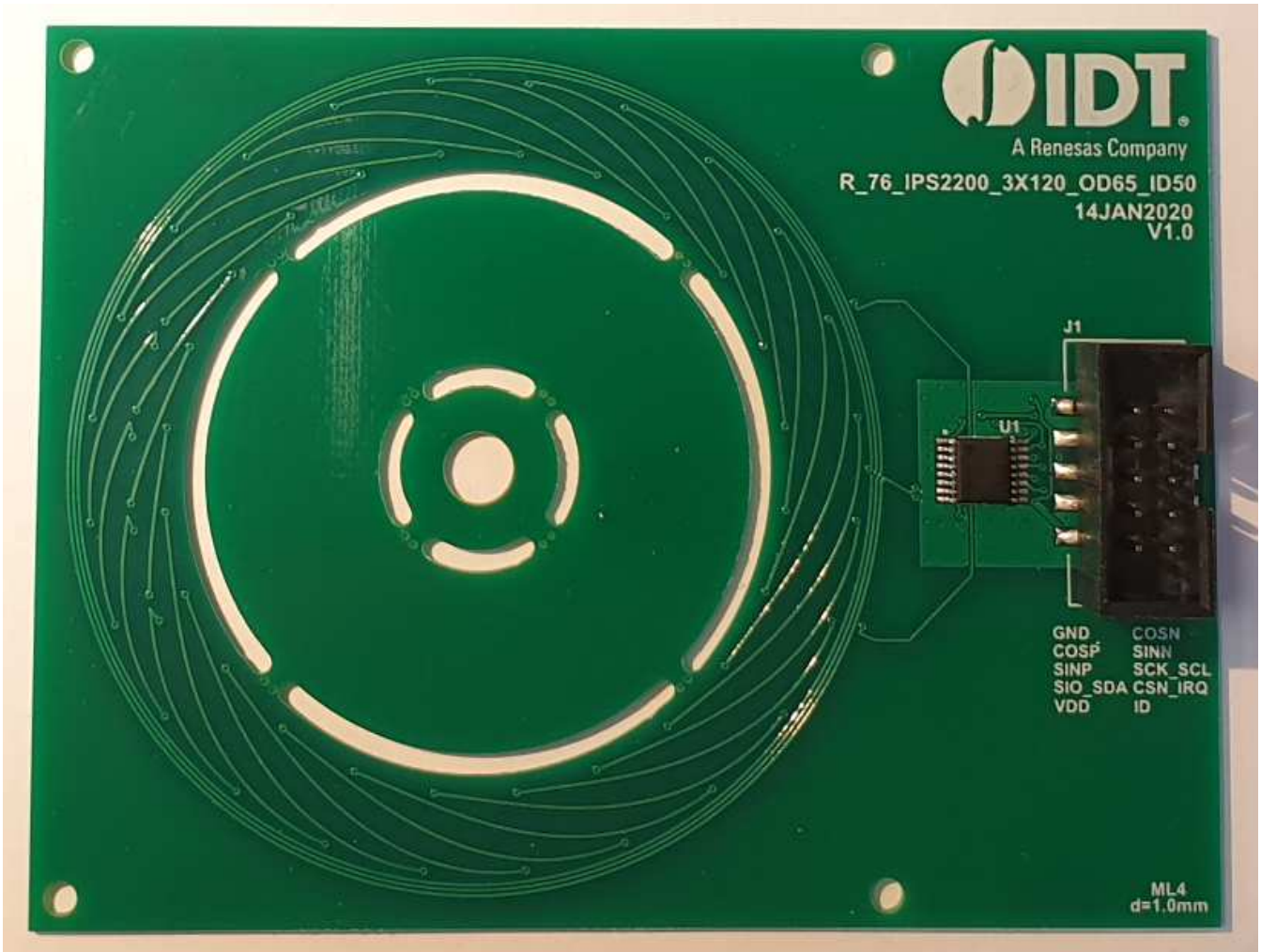
Figure 1. Sensor Board
