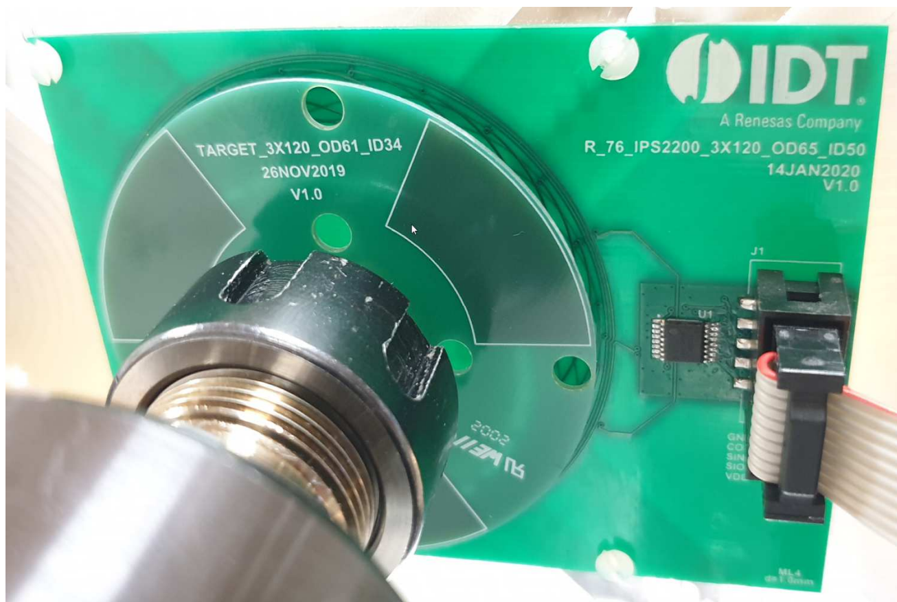
Figure 3. Setup
