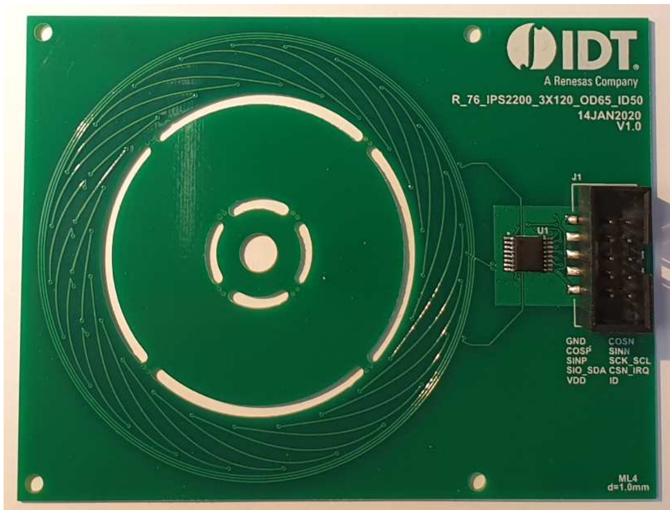
Figure 1. Sensor Board
