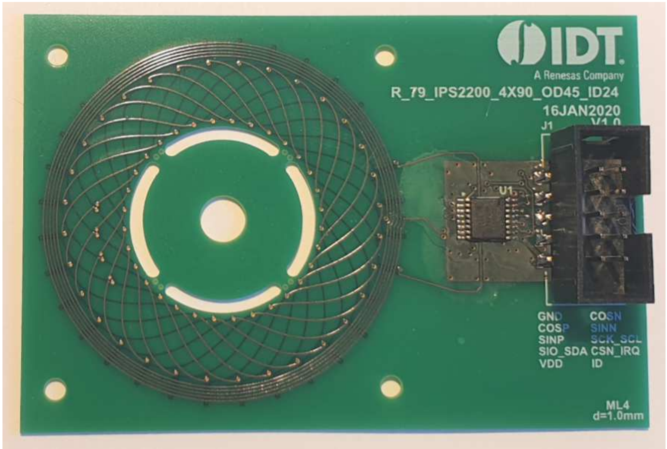
Figure 1. Sensor Board
