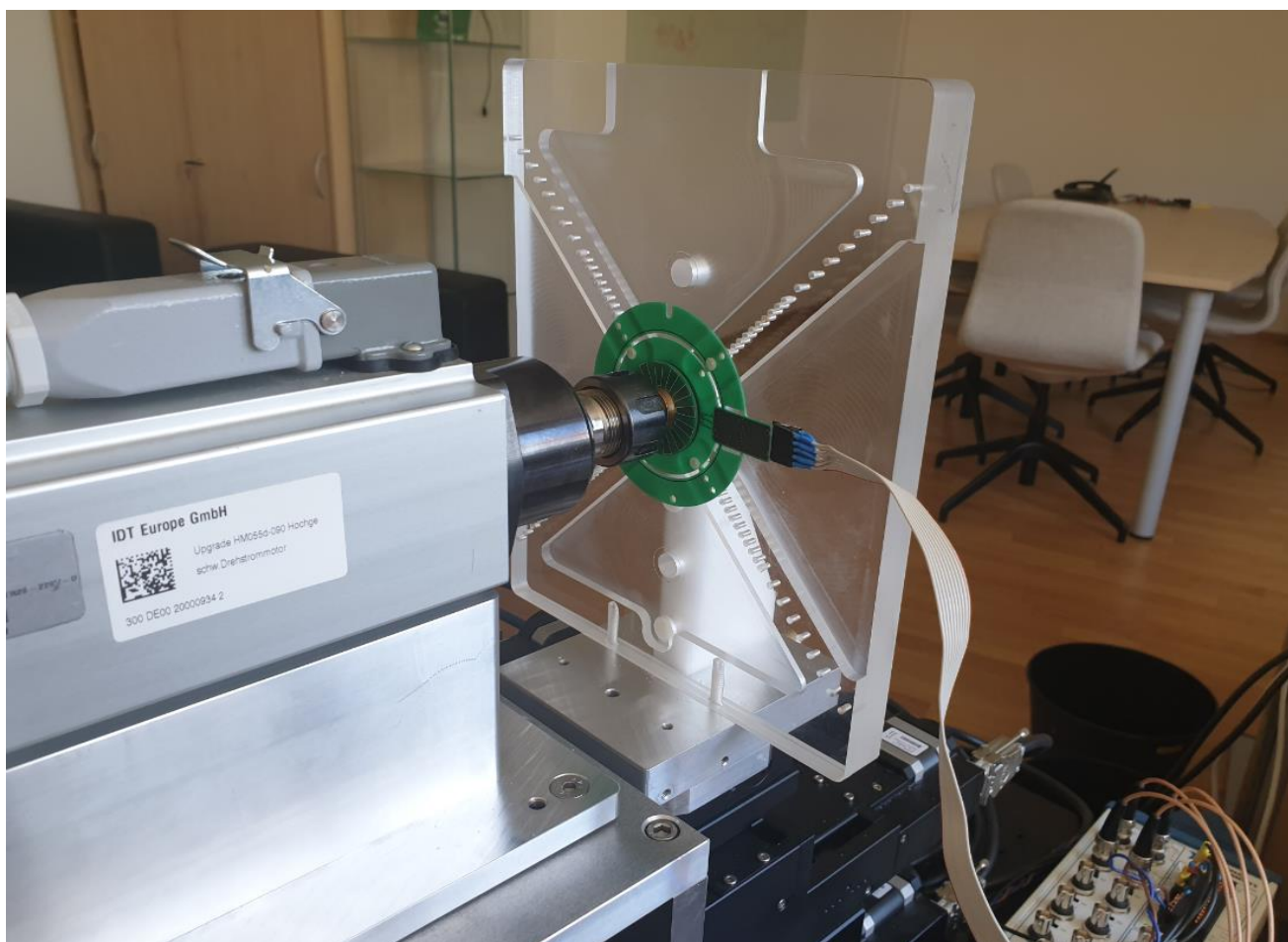
Figure 3. Setup
