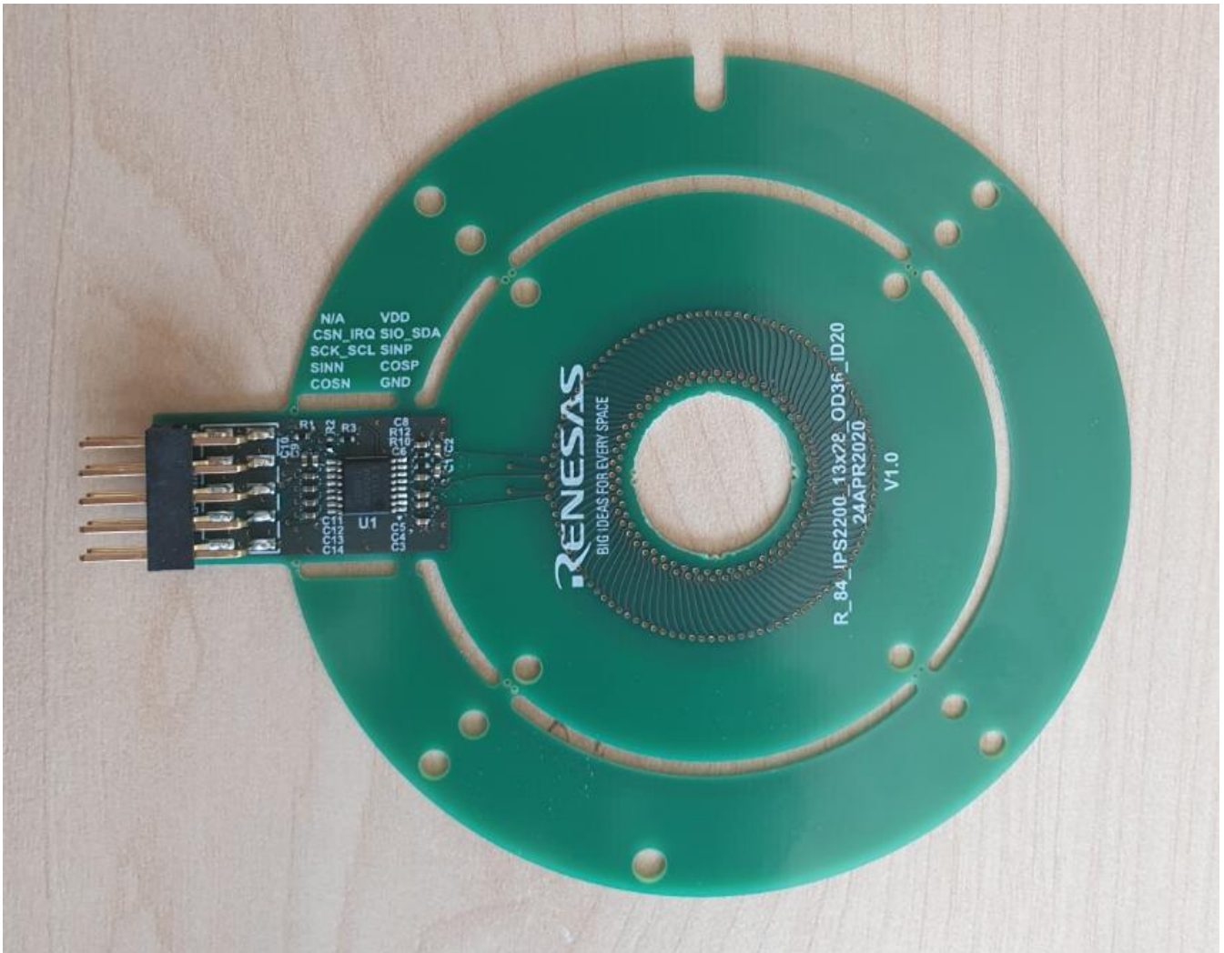
Figure 1. Sensor Board
