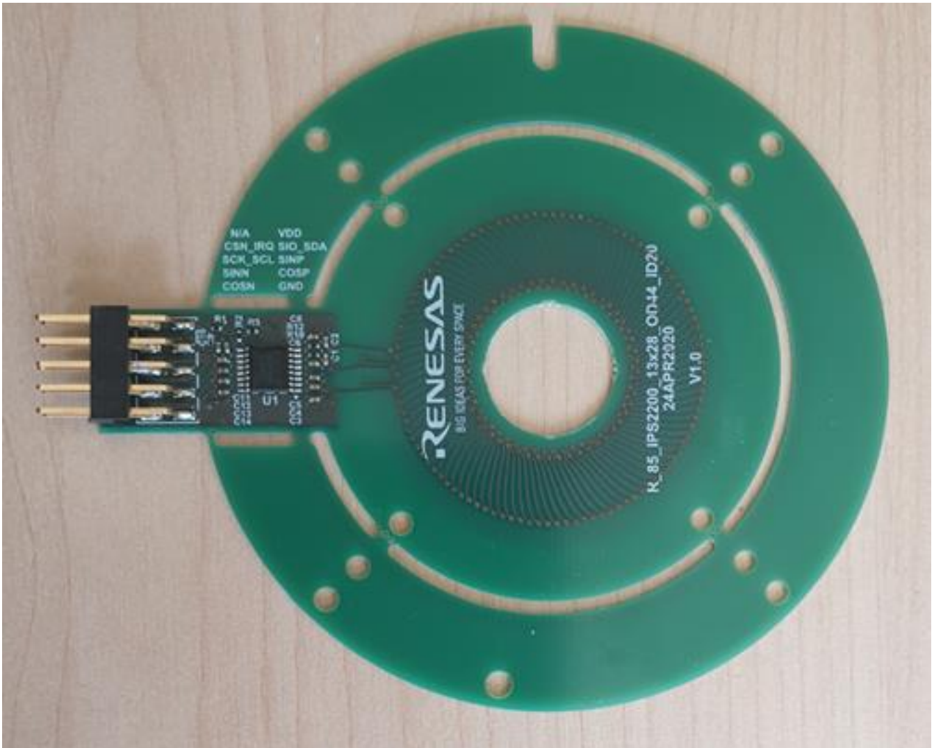
Figure 1. Sensor Board
