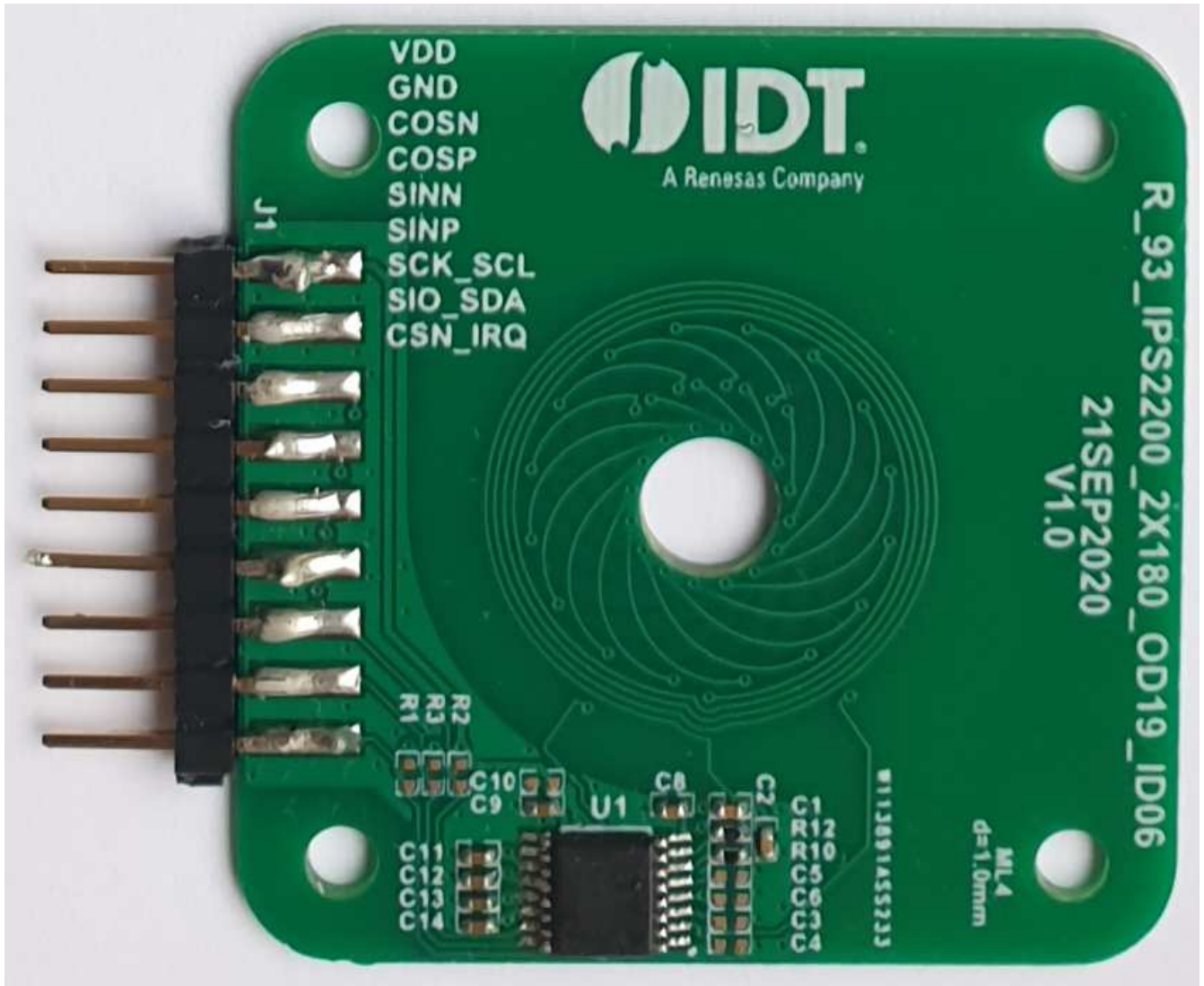
Figure 1. Sensor Board
