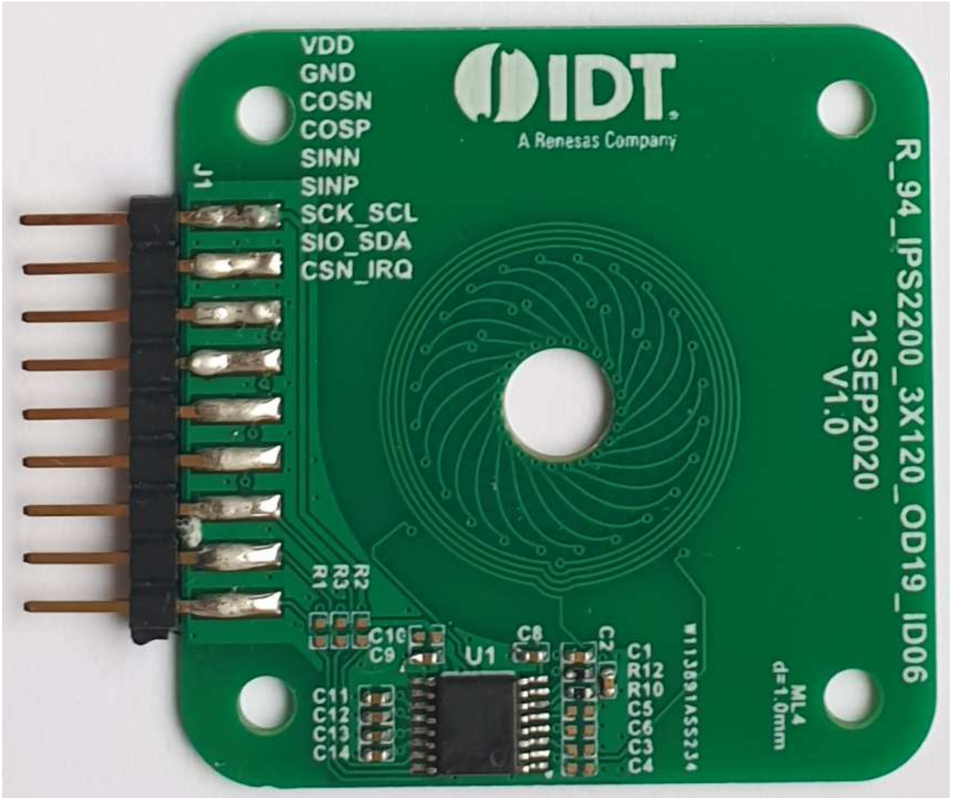
Figure 1. Sensor Board
