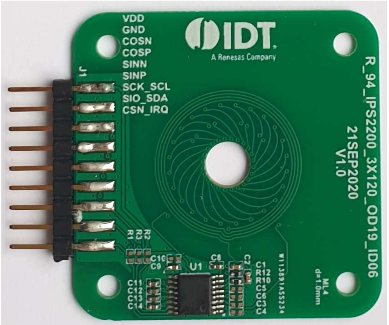
Figure 1. Sensor Board
