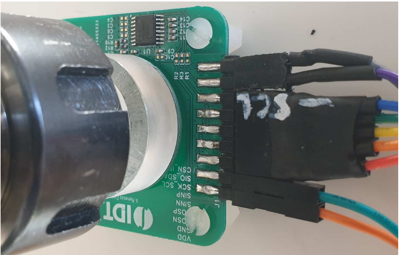
Figure 3. Setup
