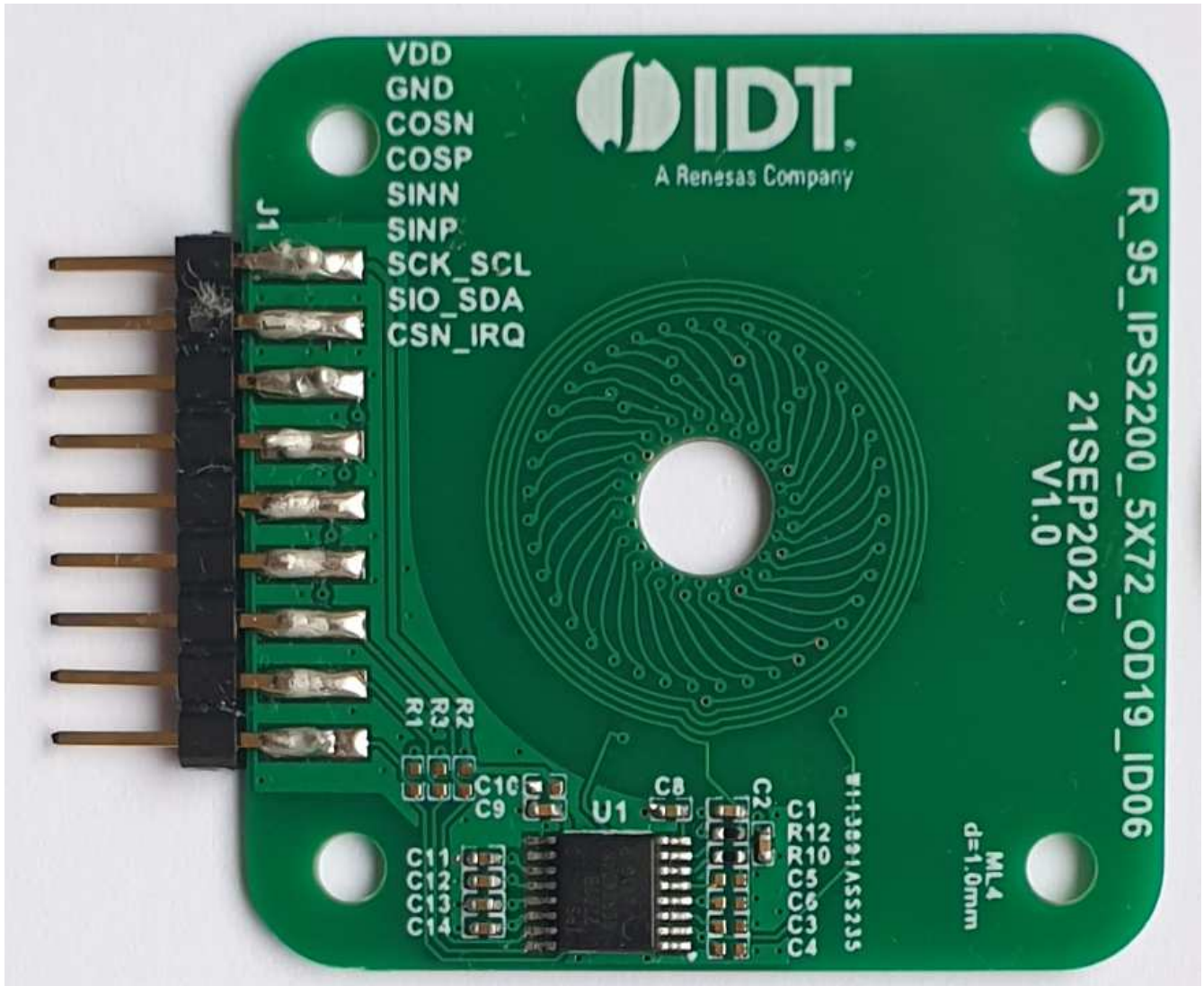
Figure 1. Sensor Board
