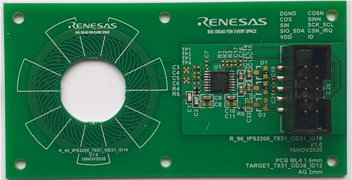
Figure 1. Sensor Board
