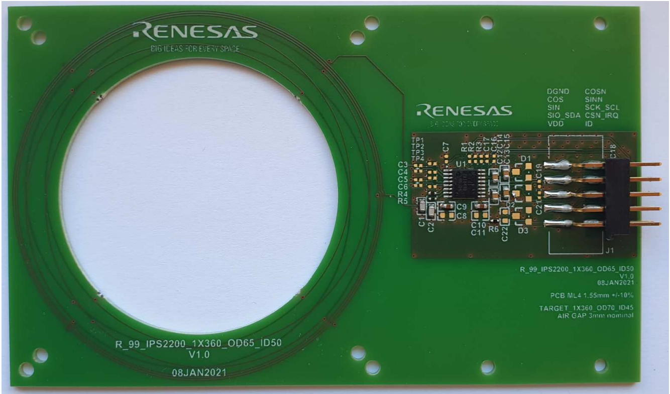
Figure 1. Sensor Board
