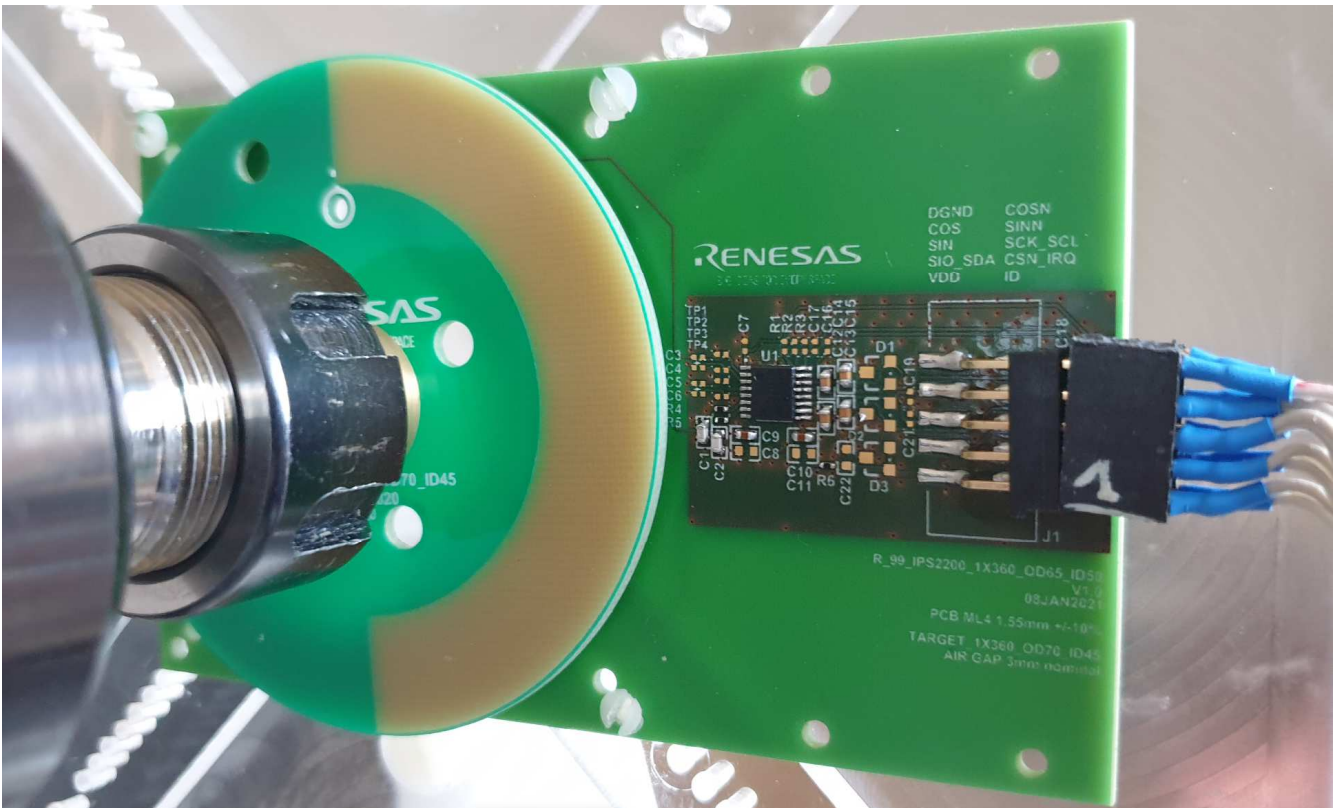
Figure 3. Setup
