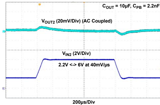
Figure 48. Line Transient Response
