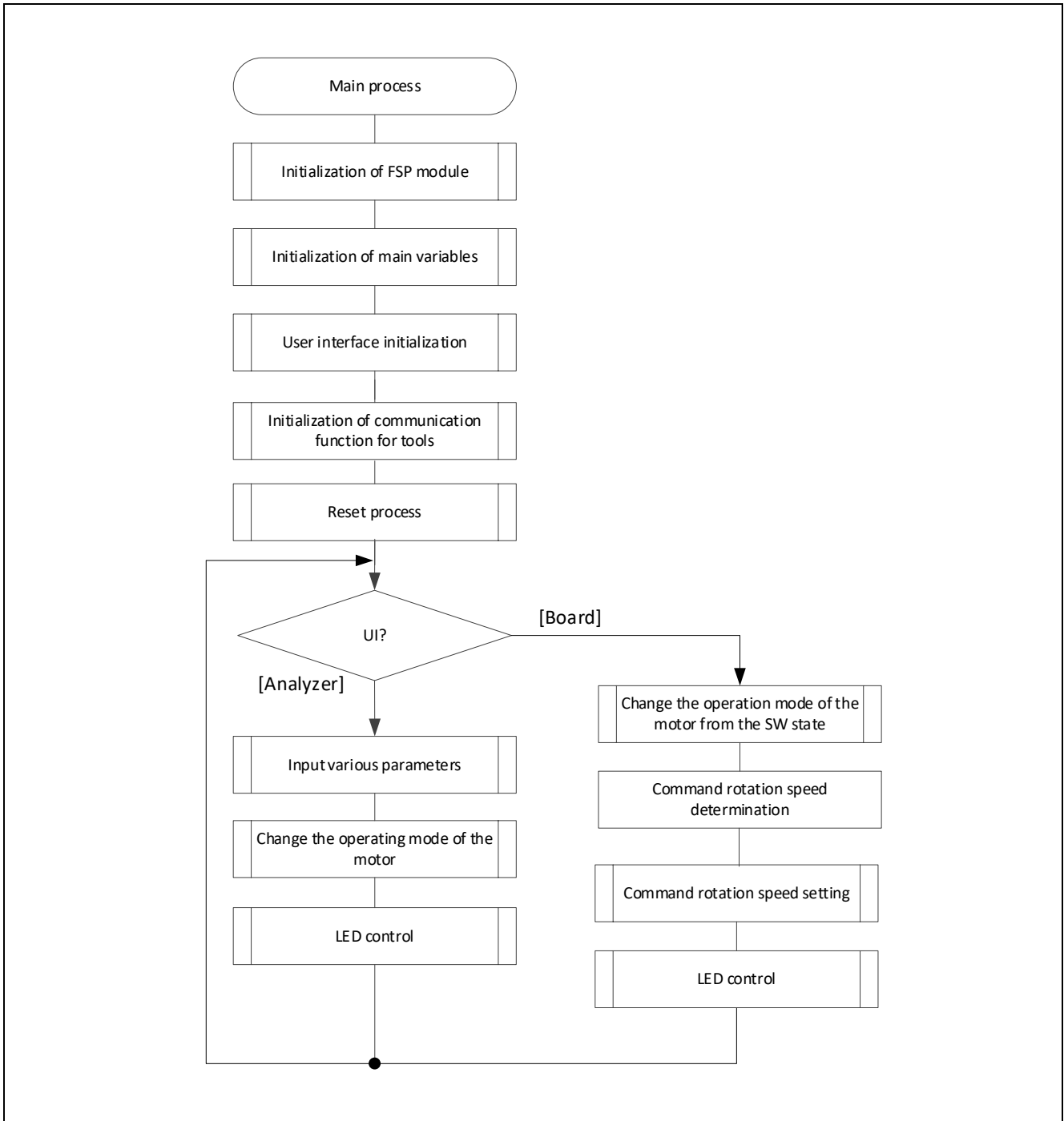
Figure 3-8 Main process Flowchart
