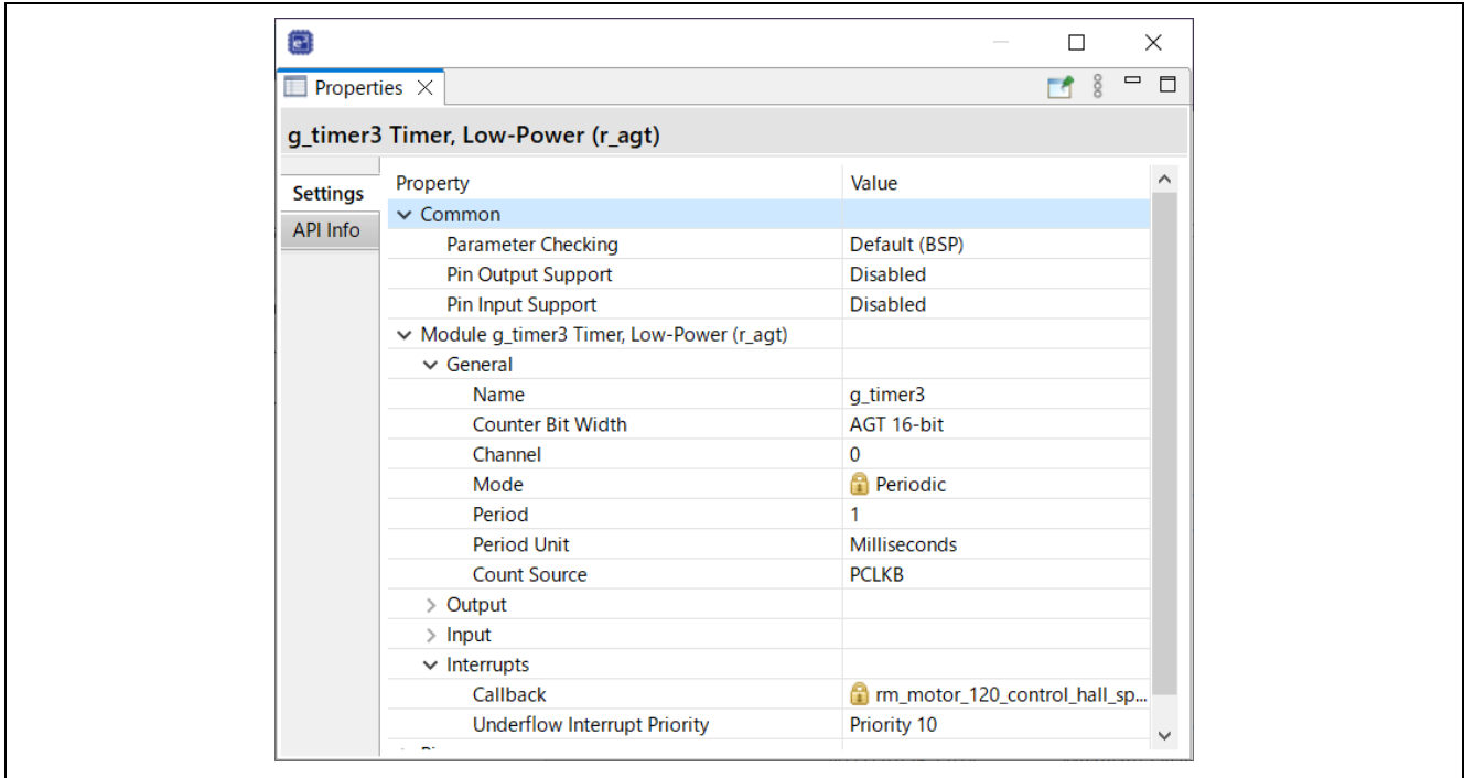
Figure 2-30 FSP configuration of AGT driver
