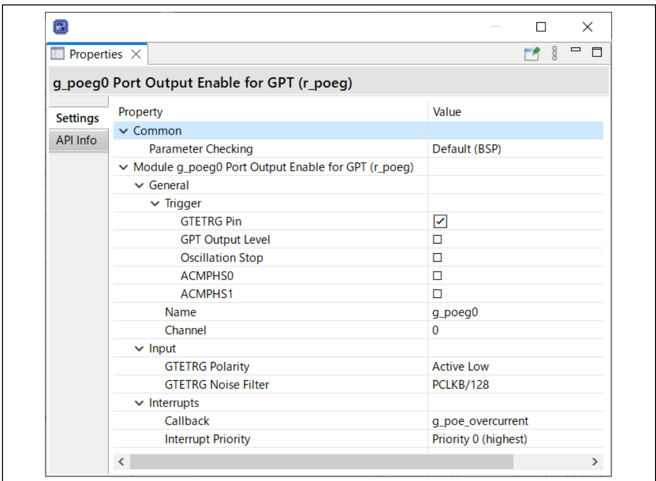
Figure 2-33 FSP configuration of POEG driver
