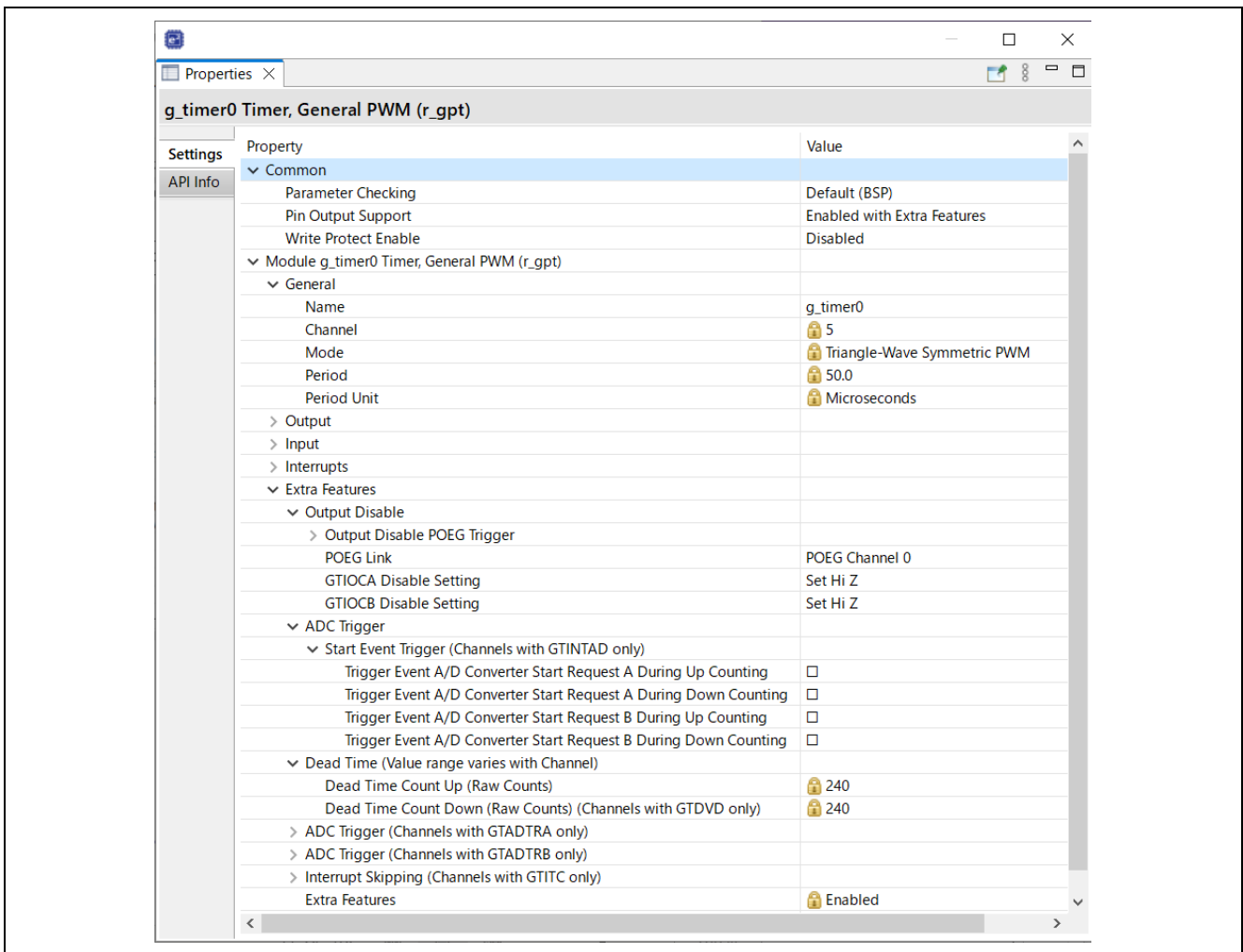
Figure 2-31 FSP configuration of GPT driver(complementary PWM output)
