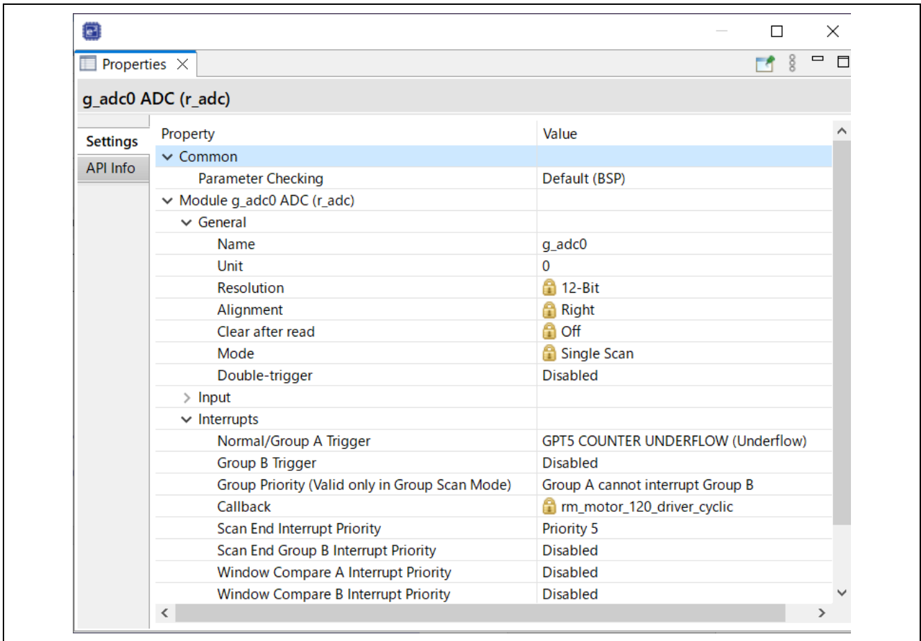
Figure 2-28 FSP configuration of ADC driver [1/2]
