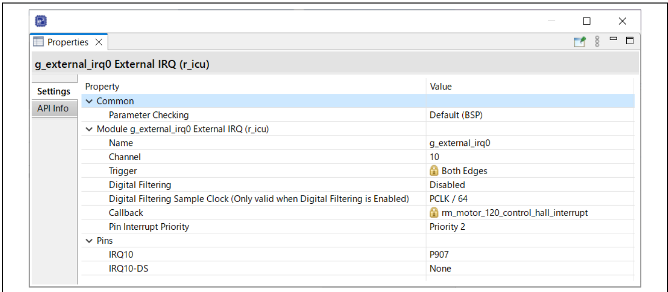
Figure 2-34 FSP configuration of IRQ driver
