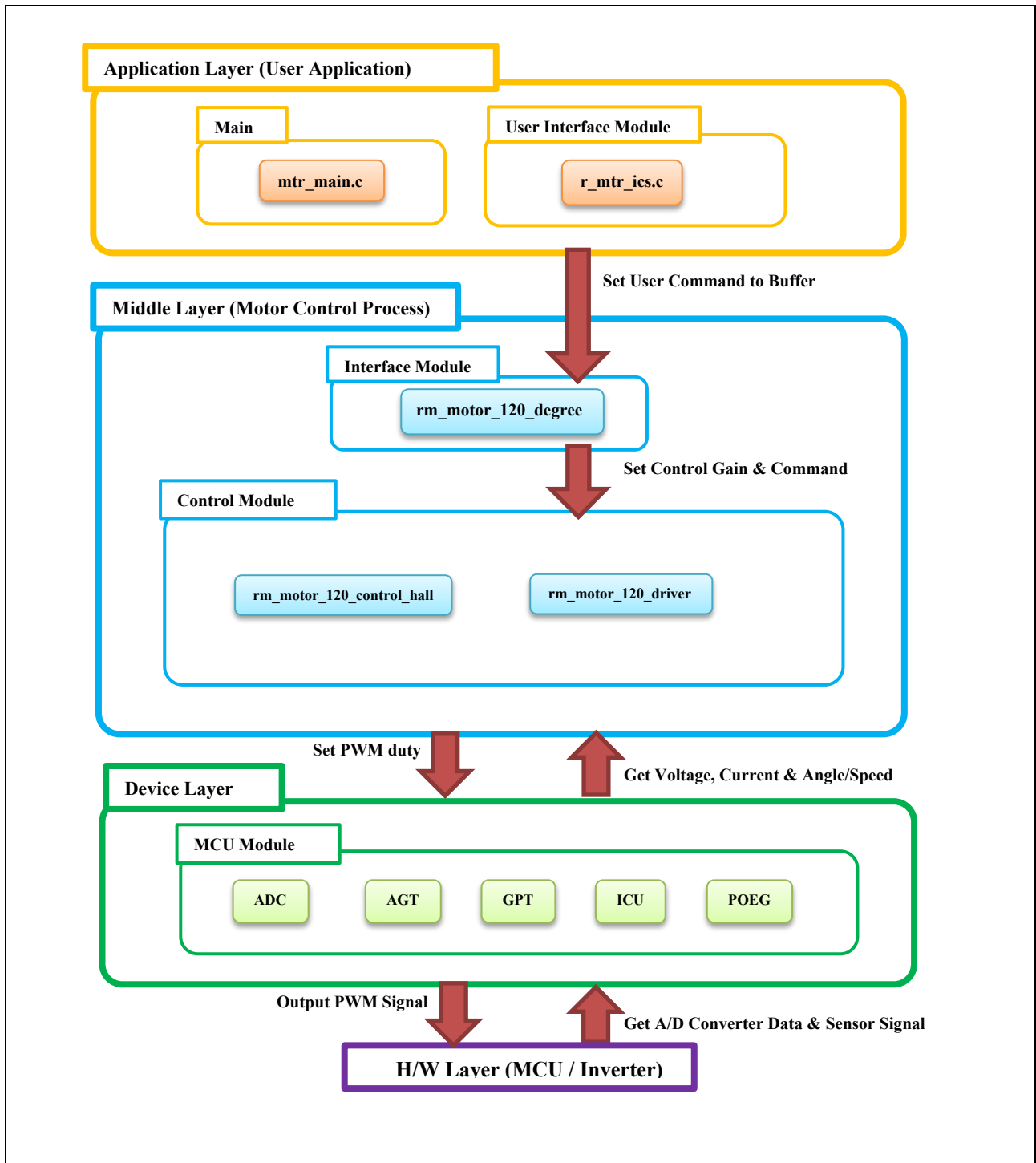
Figure 2-35 Module Configuration
