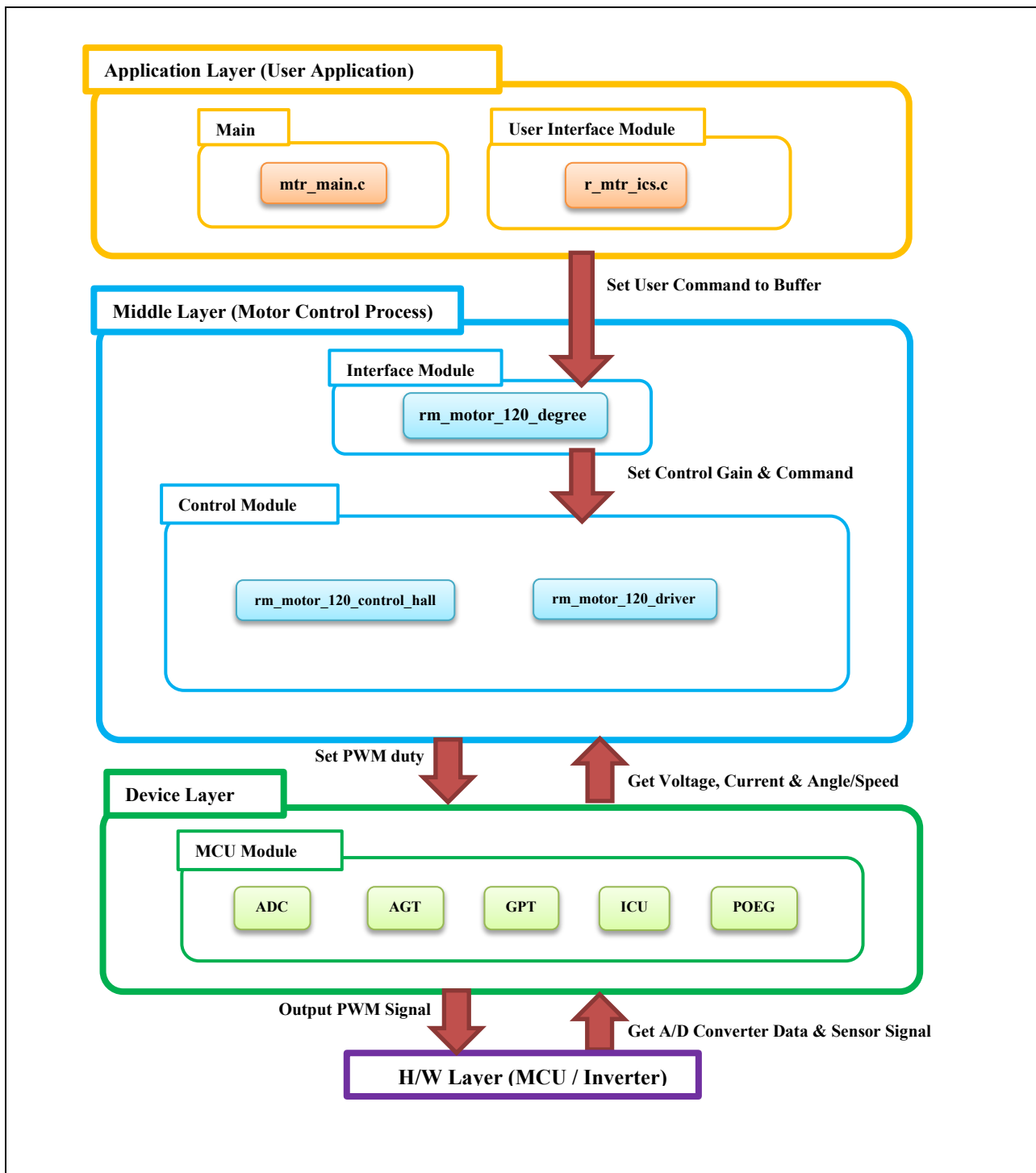
Figure 2-35 Module Configuration
