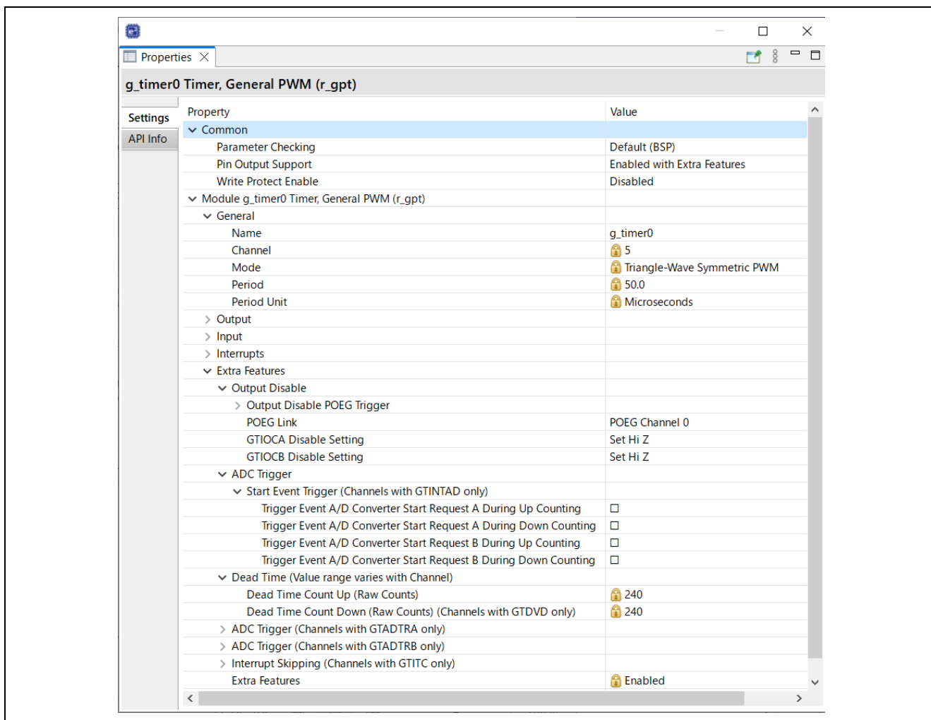
Figure 2-31 FSP configuration of GPT driver(complementary PWM output)
