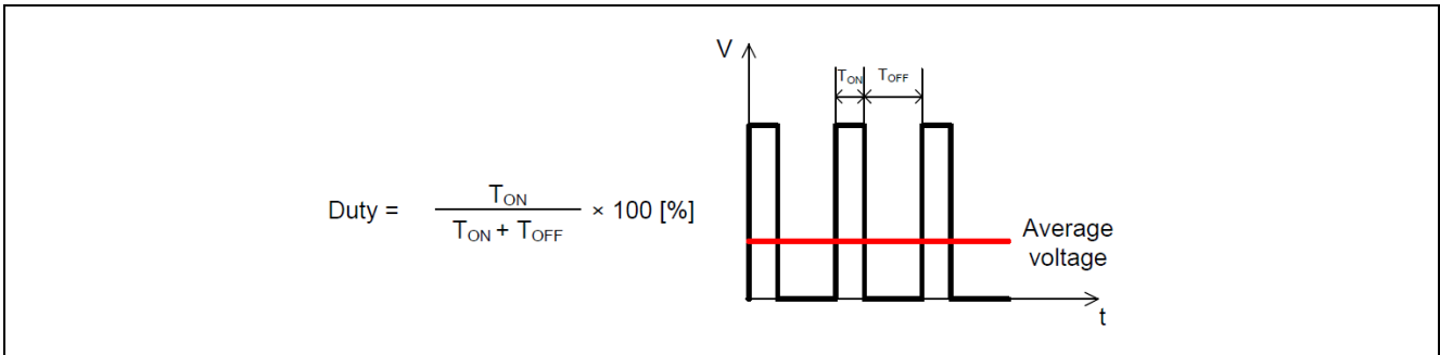
Figure 3-2 PWM Control
