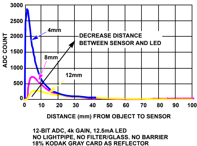
FIGURE 7. PROXIMITY SENSOR OUTPUT VARYING THE DISTANCE BETWEEN THE SENSOR AND LED
