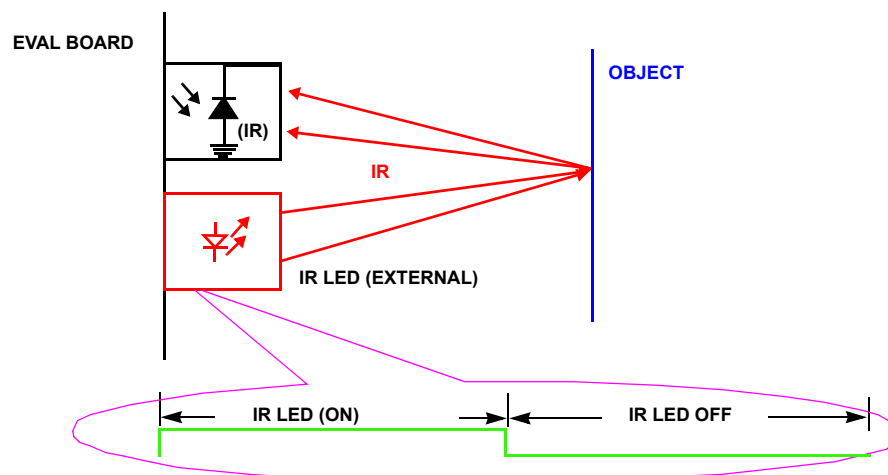
FIGURE 4B. SENSING OBJECT WITHIN 10CM FOR PROXIMITY DETECTION
