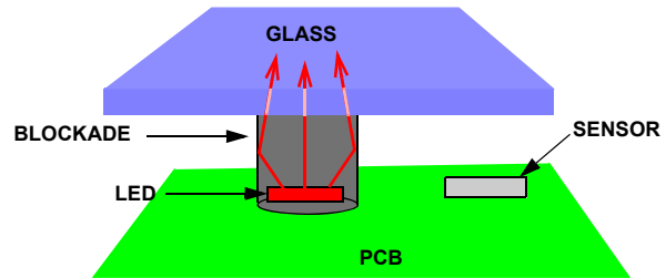
FIGURE 17. DIAGRAM OF PROXIMITY SET-UP HIGHLIGHTING A CIRCULAR BARRIER SURROUNDING THE LED
