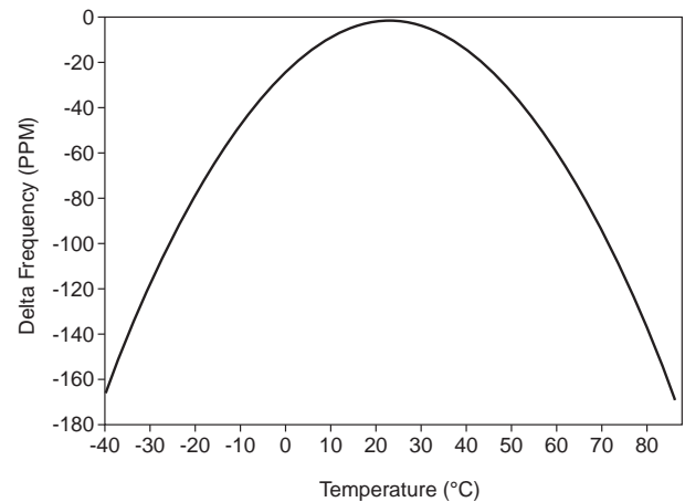
FIGURE 2. CRYSTAL FREQUENCY DEVIATION vs TEMPERATURE
