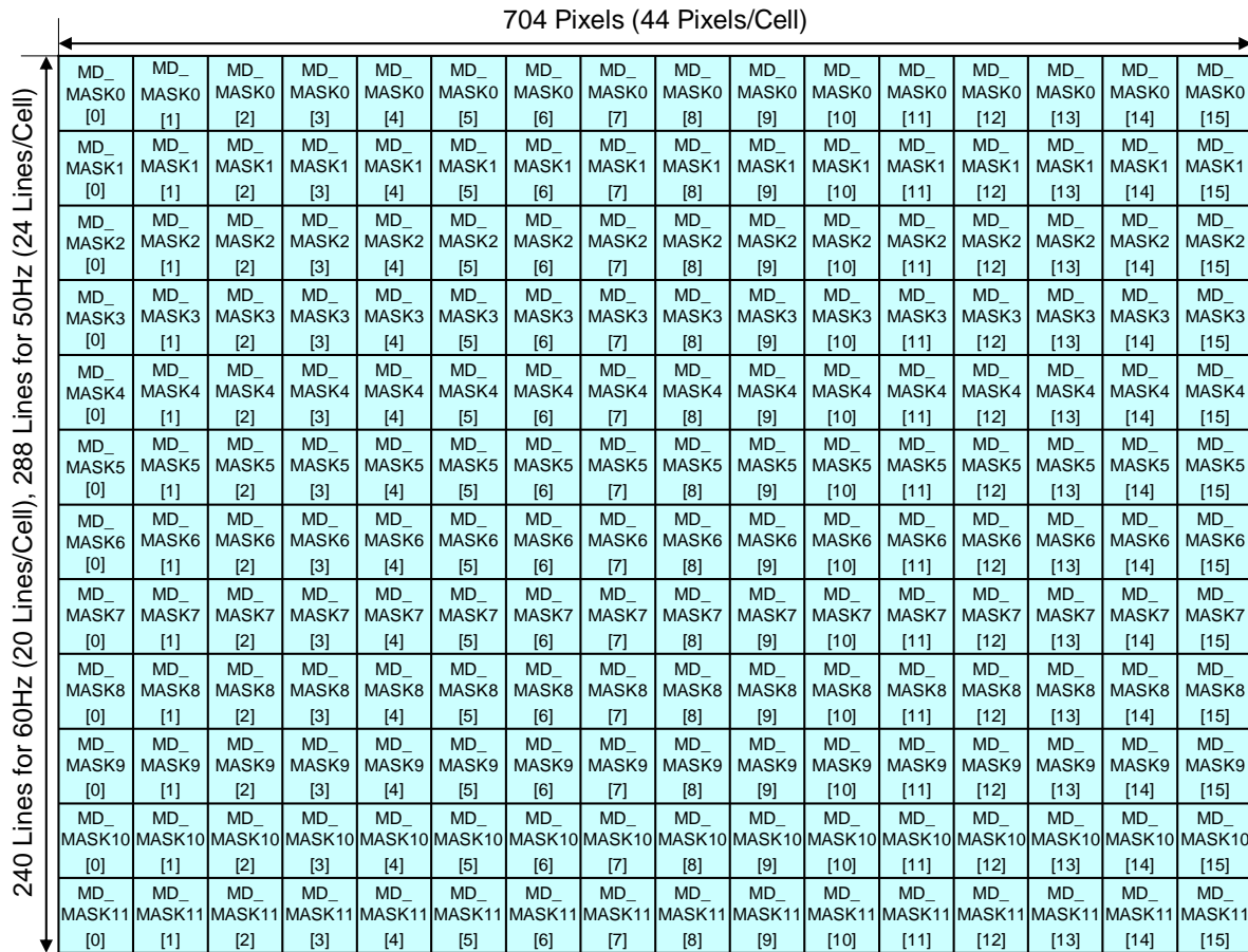
MOTION DETECTION MASK AND CELL DEFINITION
