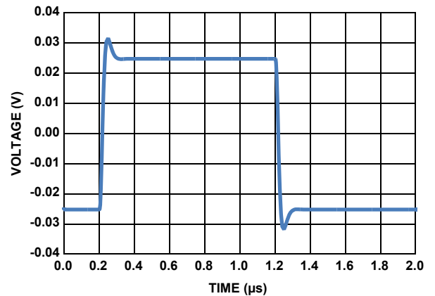
FIGURE 7. SIMULATED SMALL SIGNAL RESPONSE
