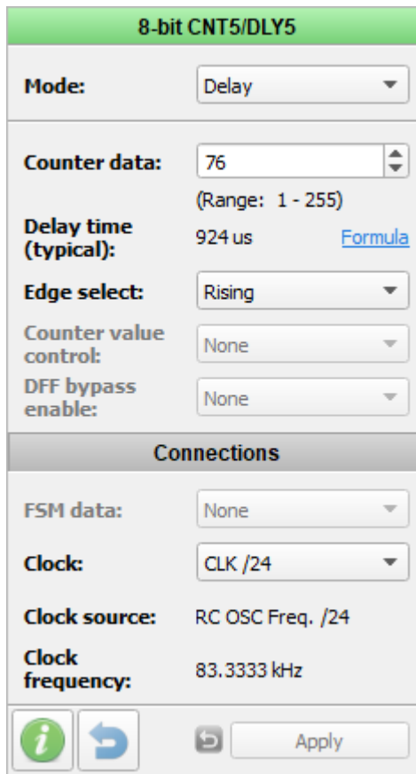
Figure 18: CNT5 Configuration
