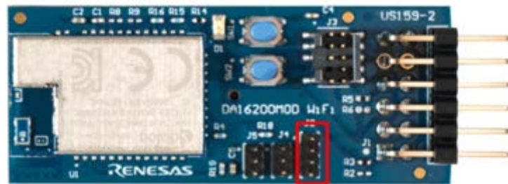
Figure 8. US159-DA16200EVZ Board
