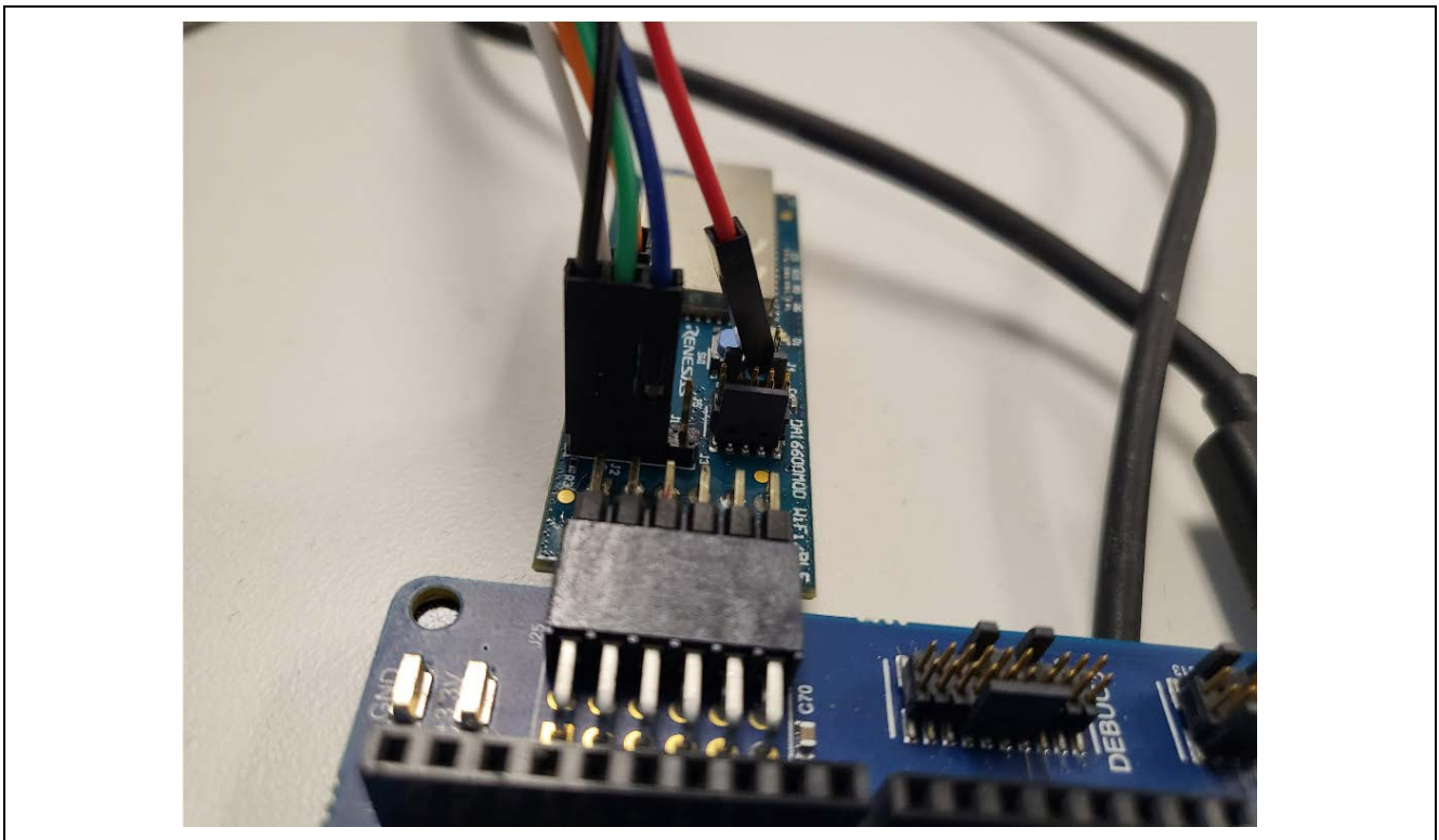
Figure 3. DA16600 Pin Connections
