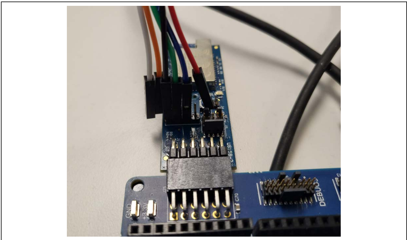
Figure 10. DA16200 Pin Connections
