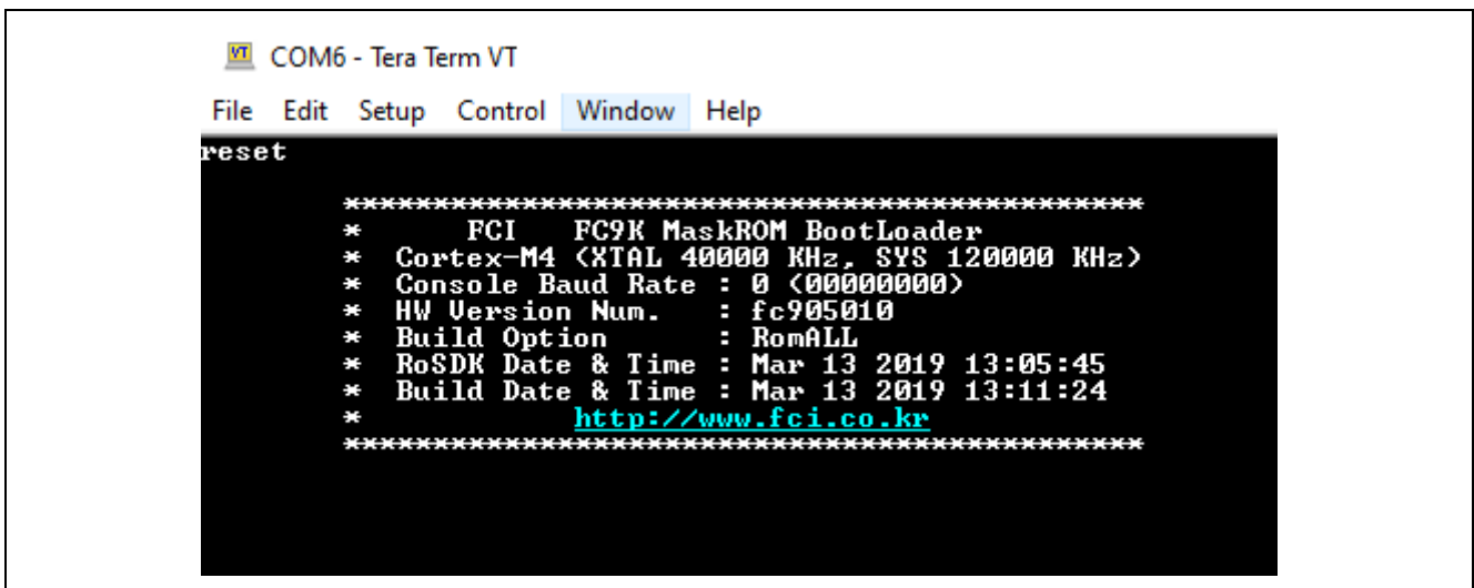
Figure 6. Bootloader Splash Screen
