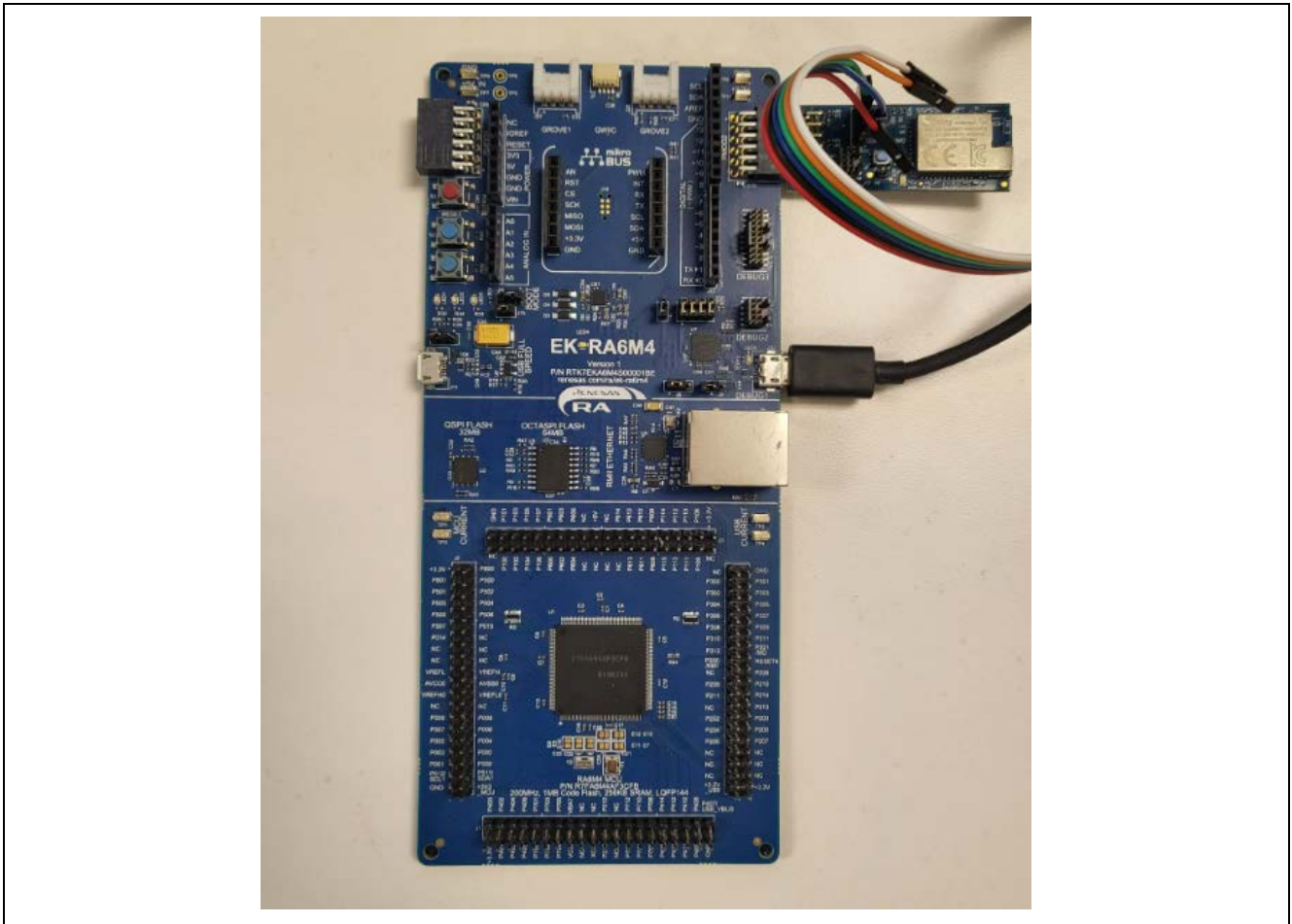
Figure 2. Pin Connections
