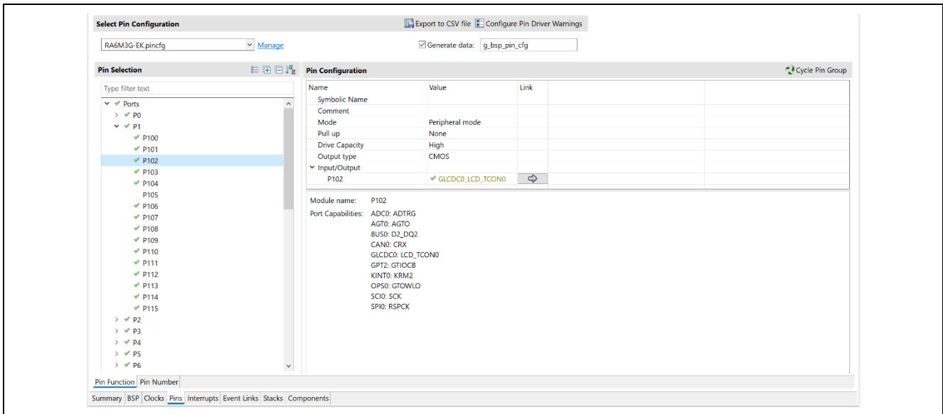
Figure 35. LCD_TCON0 Settings in Pin Selection window
