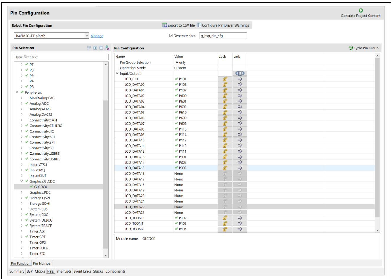
Figure 34. LCD Pin Configuration Using Configurator
