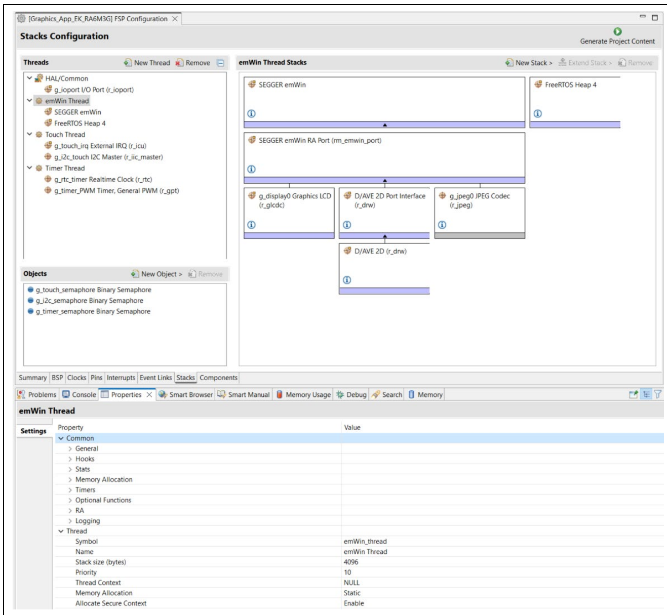
Figure 26. emWin Thread Properties and Modules Used for the Graphics Application
