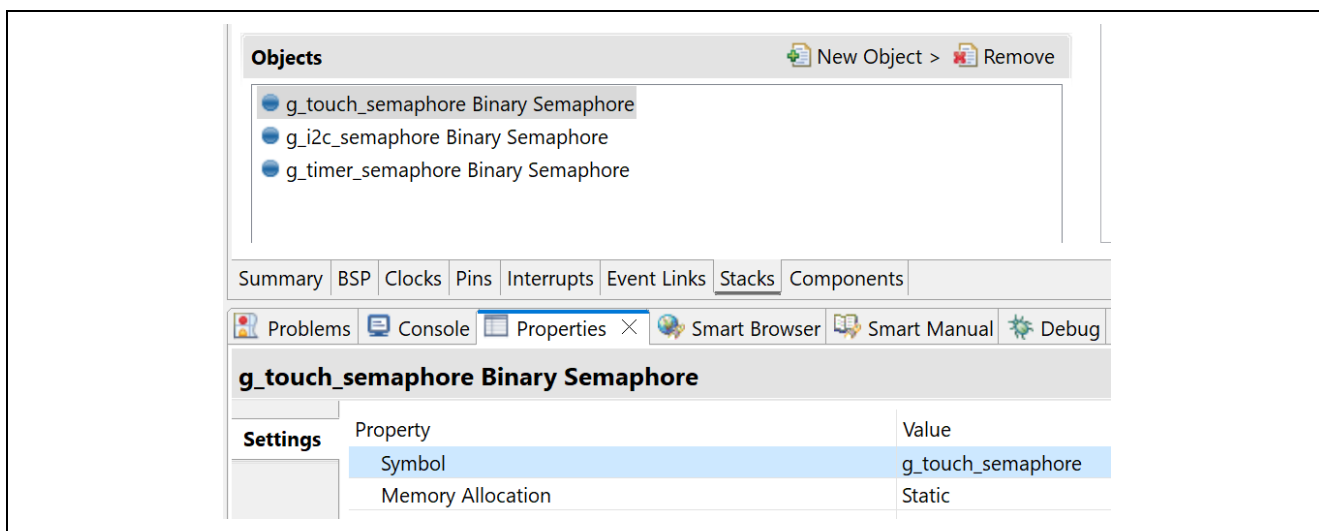
Figure 29. g_touch_semaphore Properties
