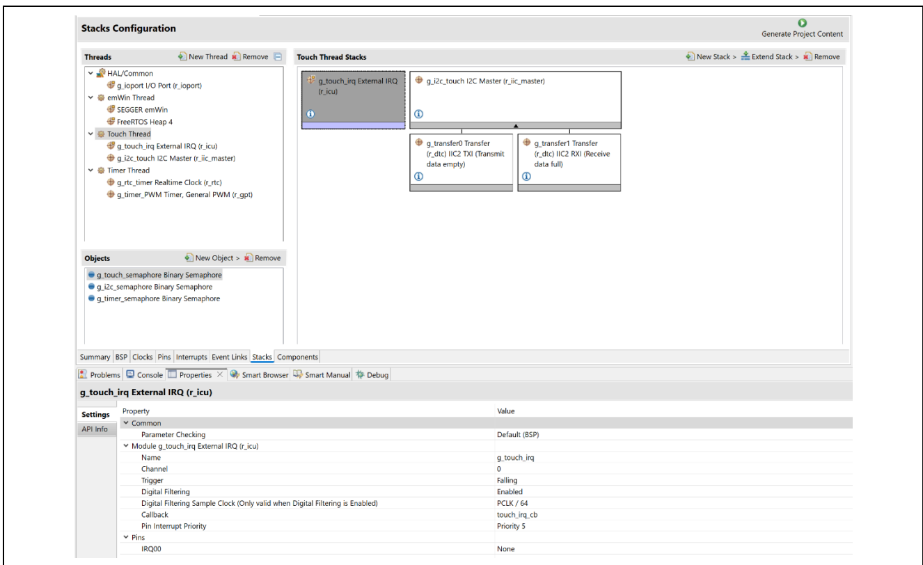
Figure 36. External Interrupt Configuration
