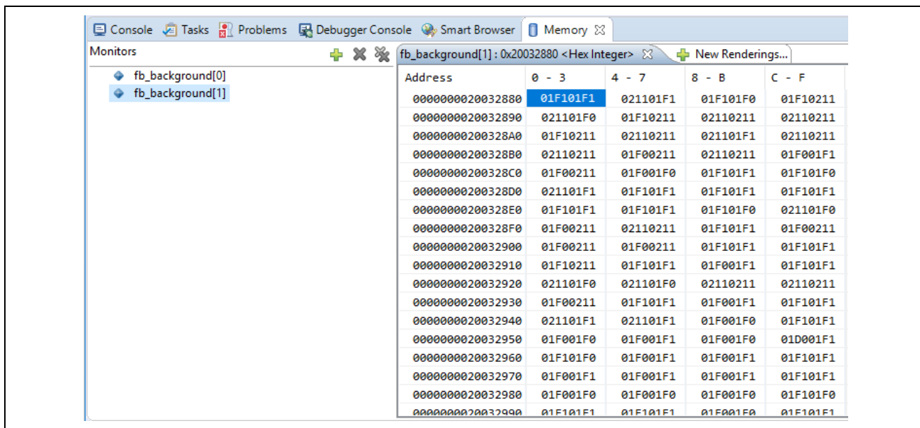
Figure 56. Framebuffer 1 Contents
