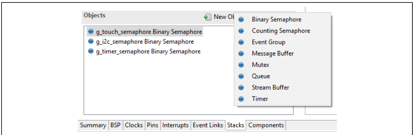
Figure 28. Objects window
