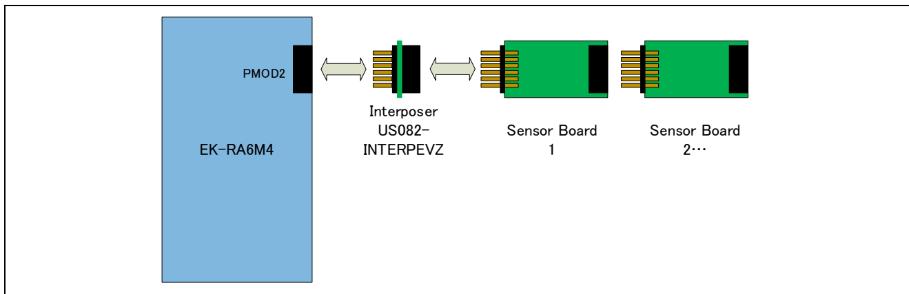
Figure 2-1 Hardware Connections for the RA6M4 Group
