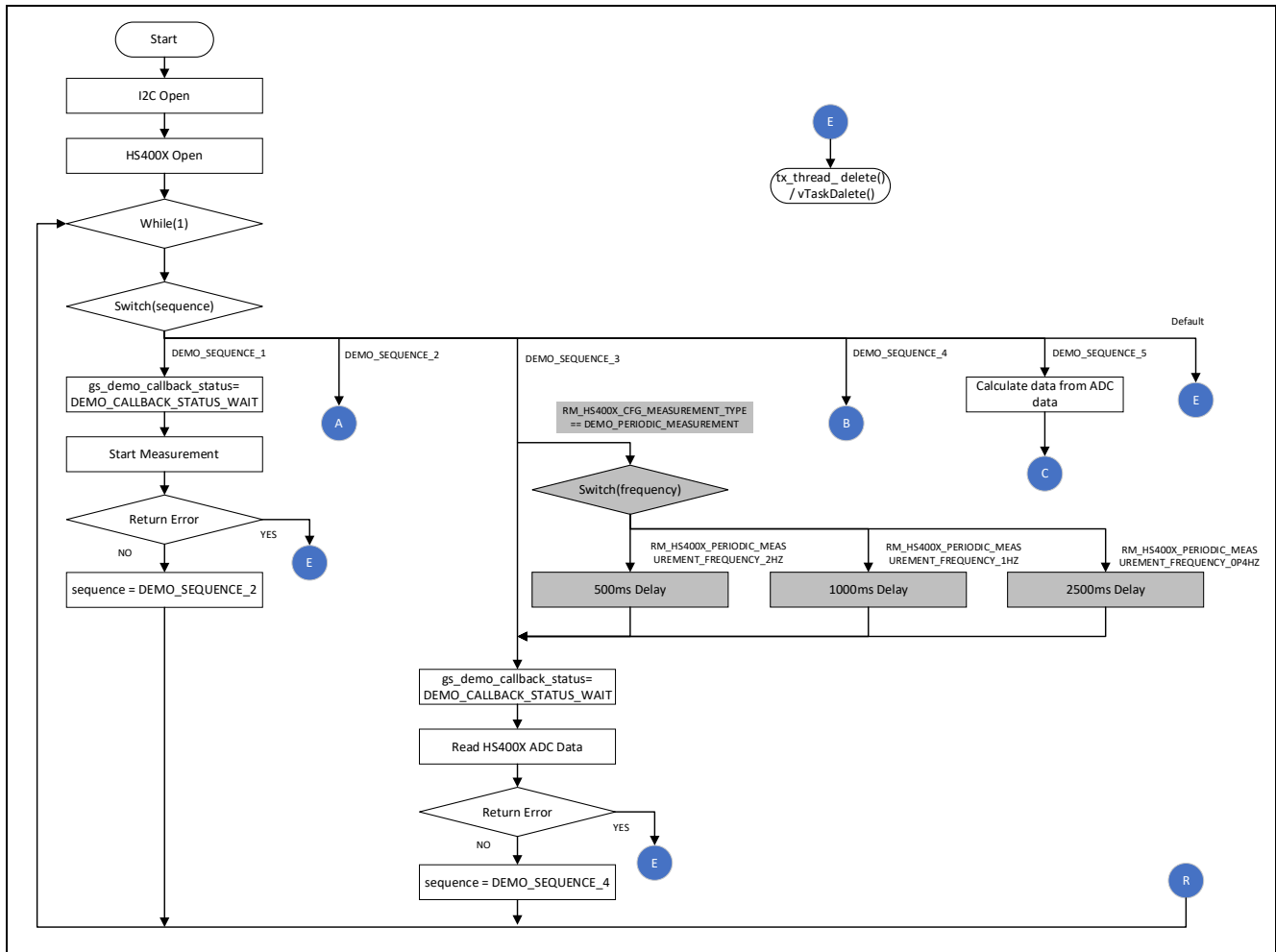
Figure 4-5 Flowchart 1 of the Main Processing in the OS Version of the Sample Software
