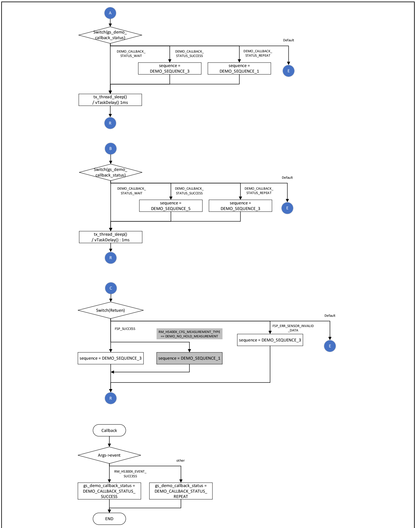
Figure 4-6 Flowchart 2 of the Main Processing in the OS Version of the Sample Software
