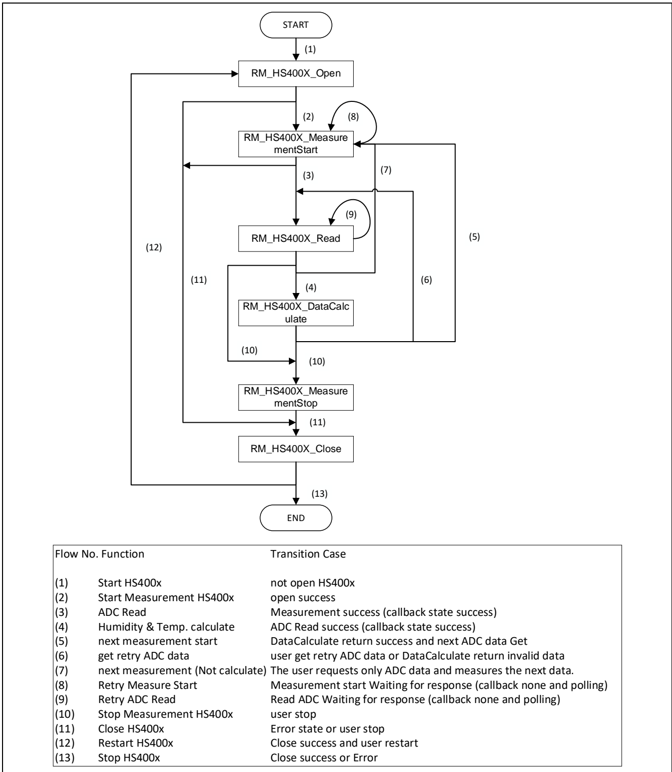
Figure 4-2 Transitions between API Function Calls
