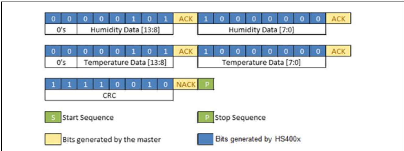
Figure 3-1 Format of I2C Communications
