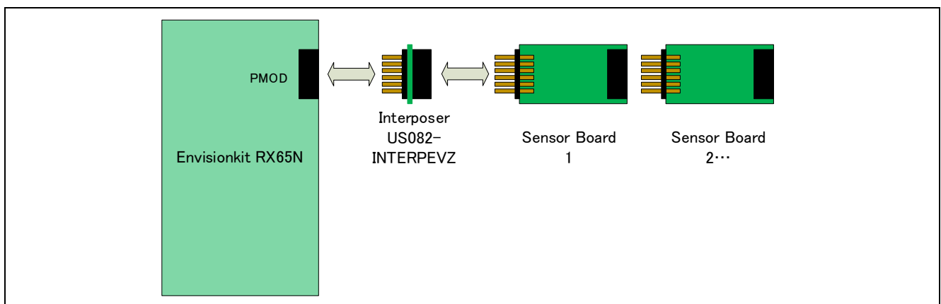
Figure 2-3 Hardware Connections for the RX Family
