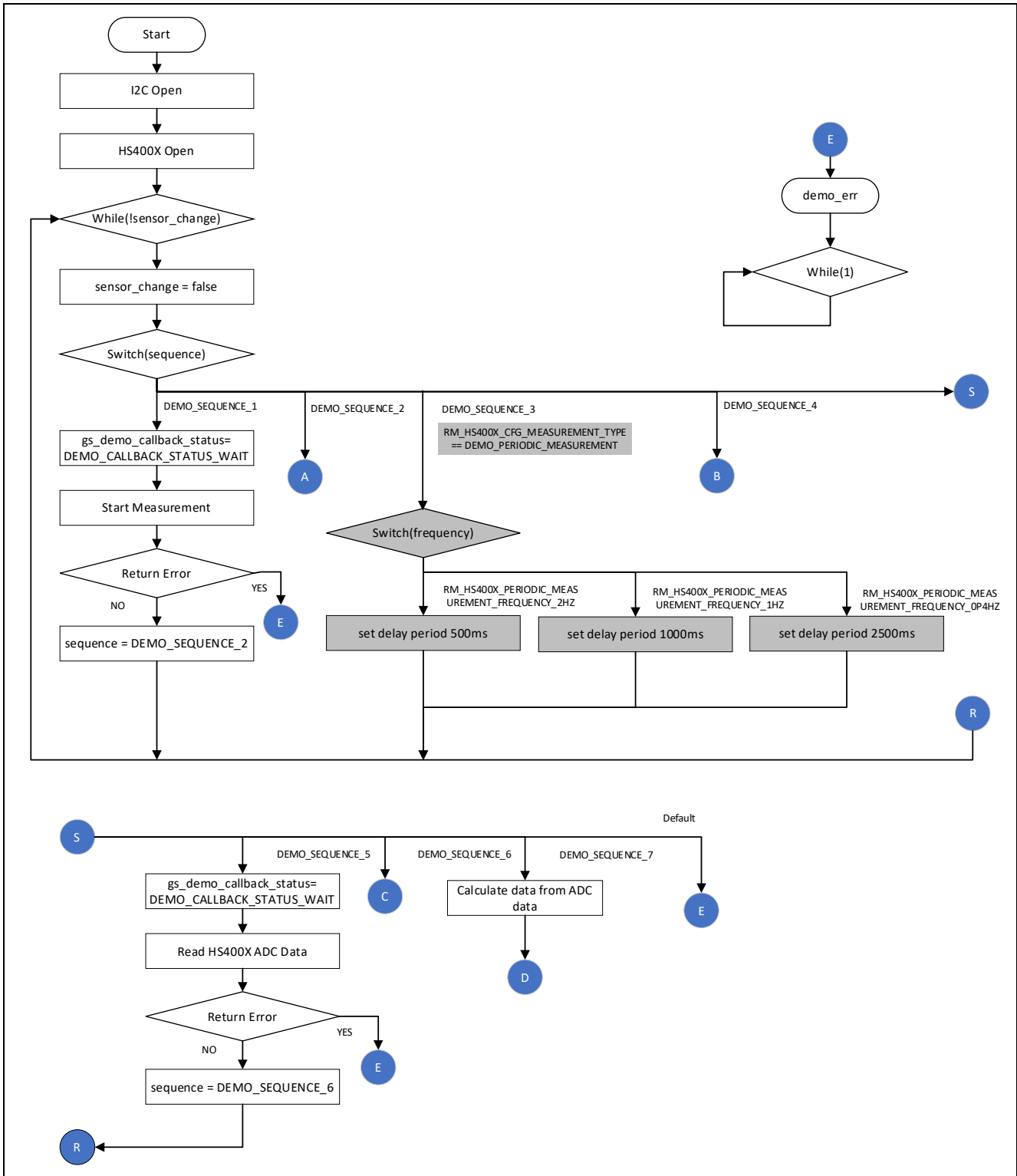
Figure 4-3 Flowchart 1 of the Main Processing in the Non-OS Version of the Sample Software
