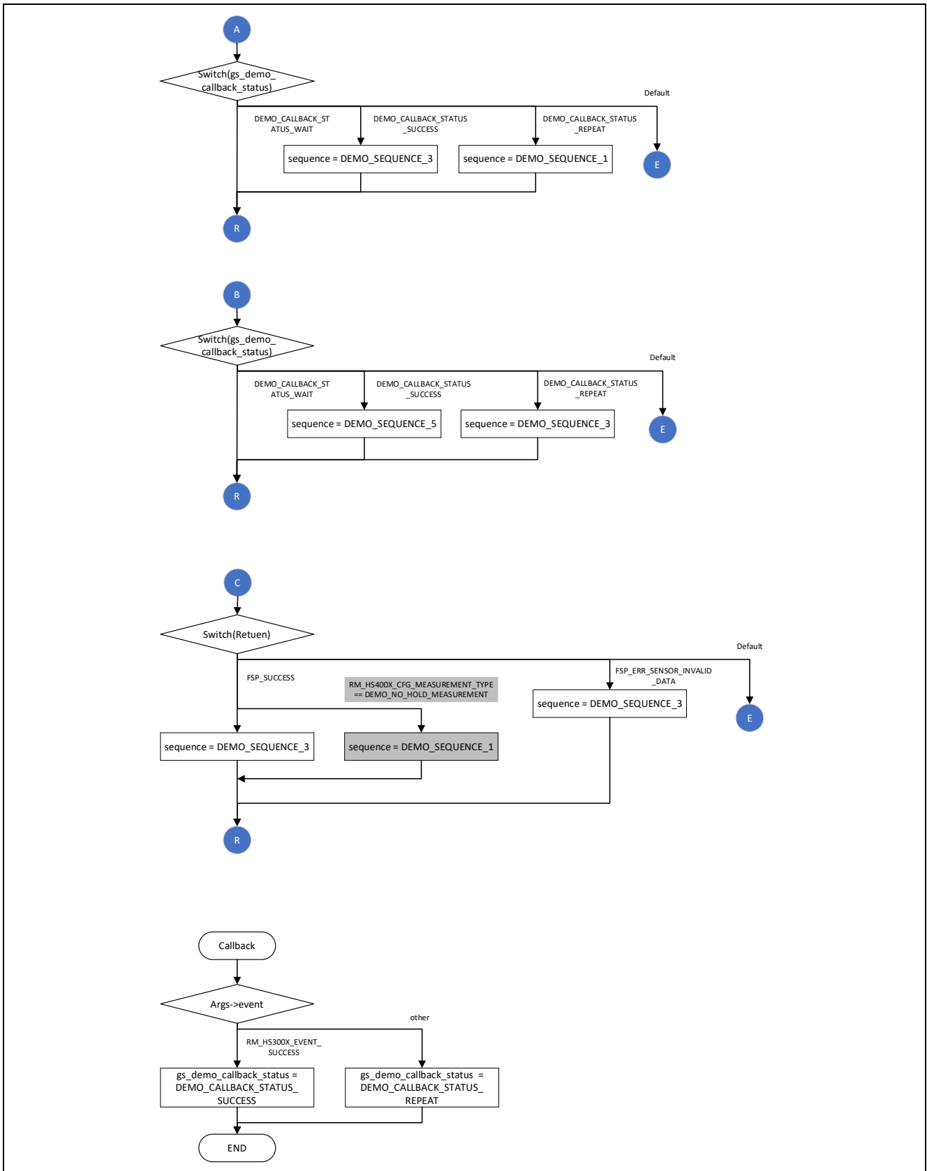
Figure 4-4 Flowchart 2 of the Main Processing in the Non-OS Version of the Sample Software
