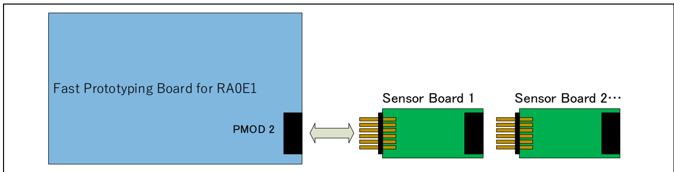
Figure 2-2 Hardware Connections for the RA0E1 Group
