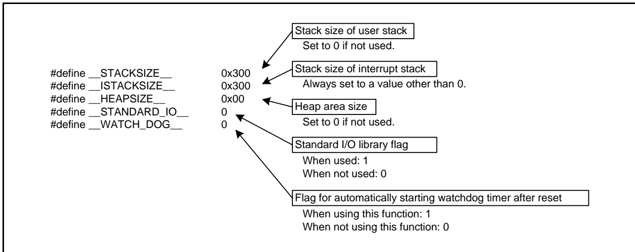
Figure 4.2 cstartdef.h
