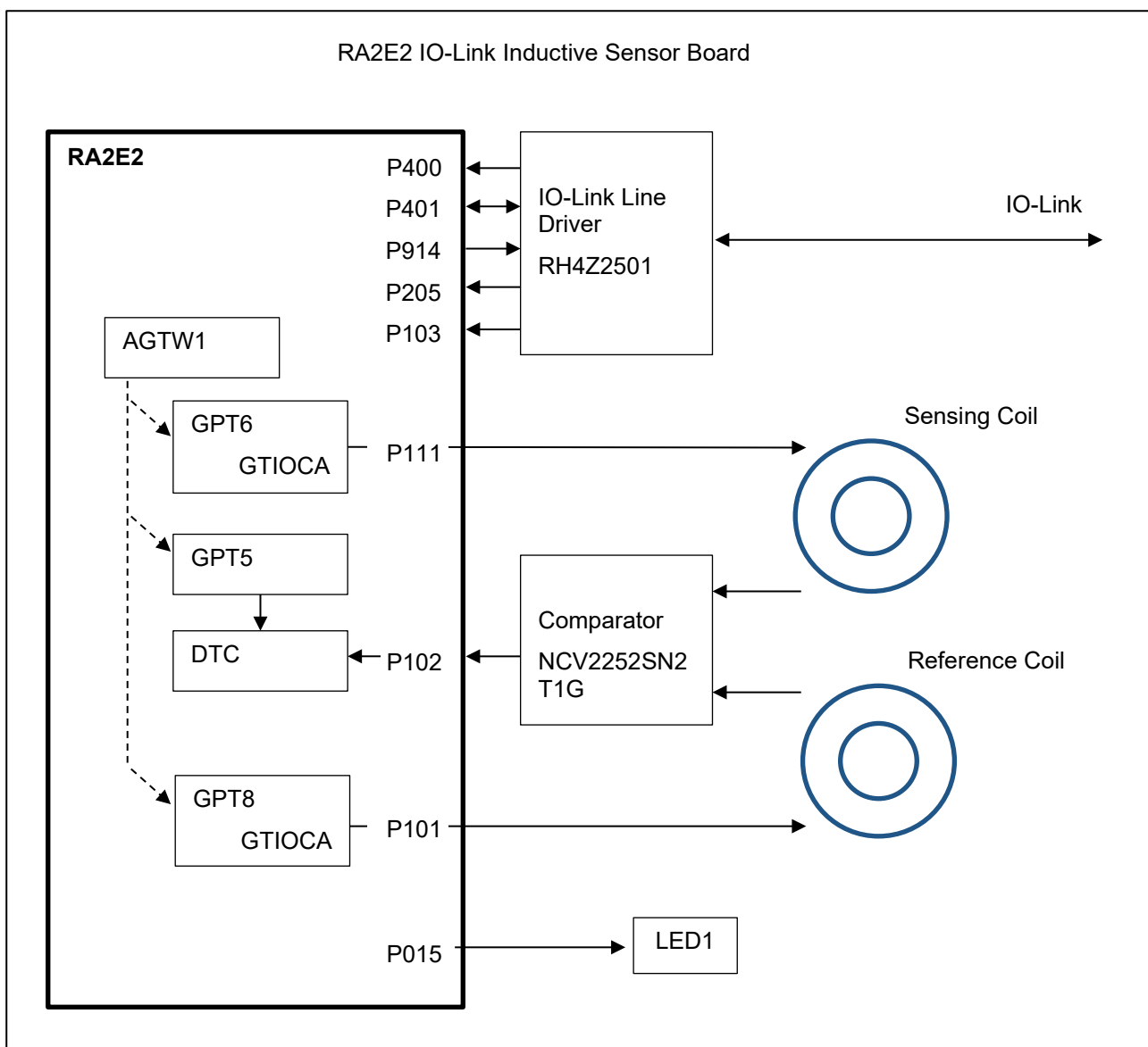
Figure 12. Peripheral Features and Terminals to be Used
