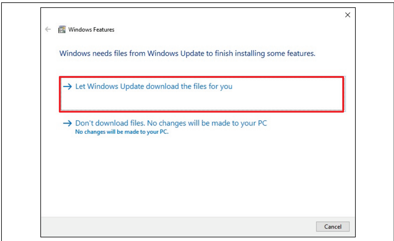
Figure 36. Windows Features
