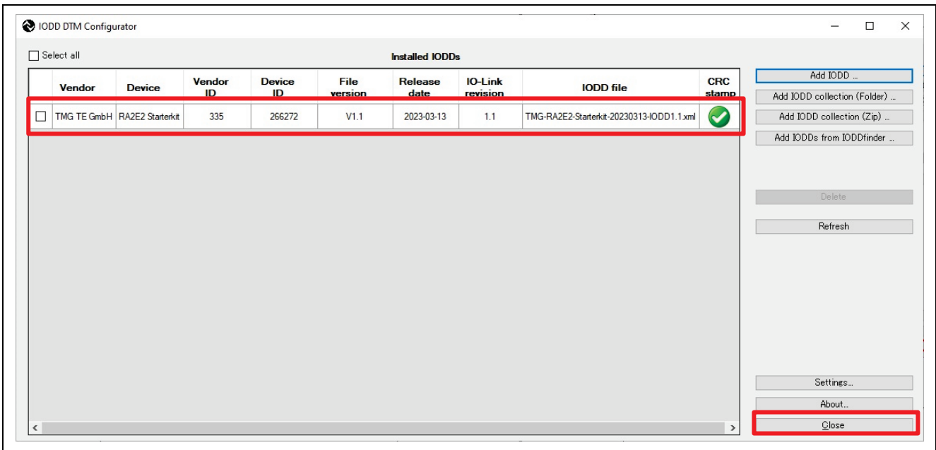
Figure 46. Installed IODDs
