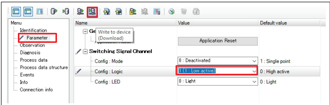
Figure 60. Config.Logic Setting
