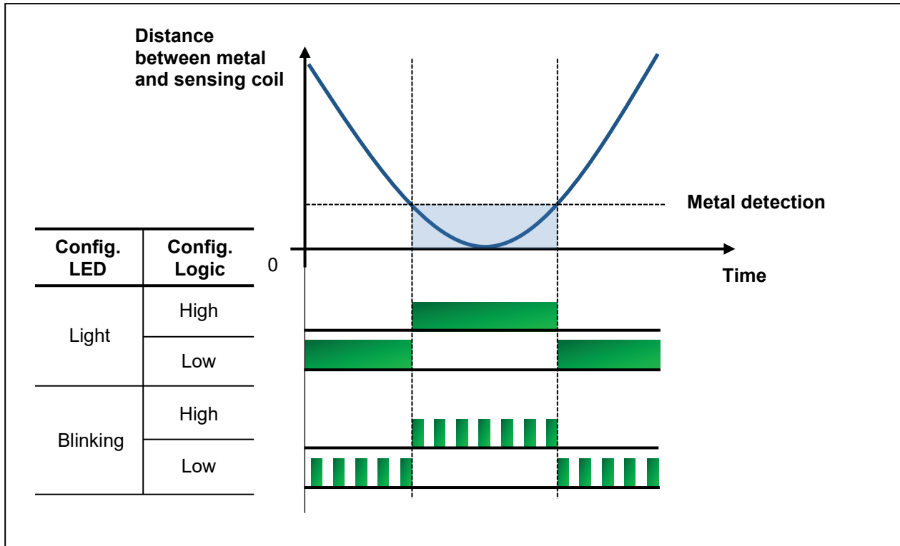
Figure 11. Image of LED Operation
