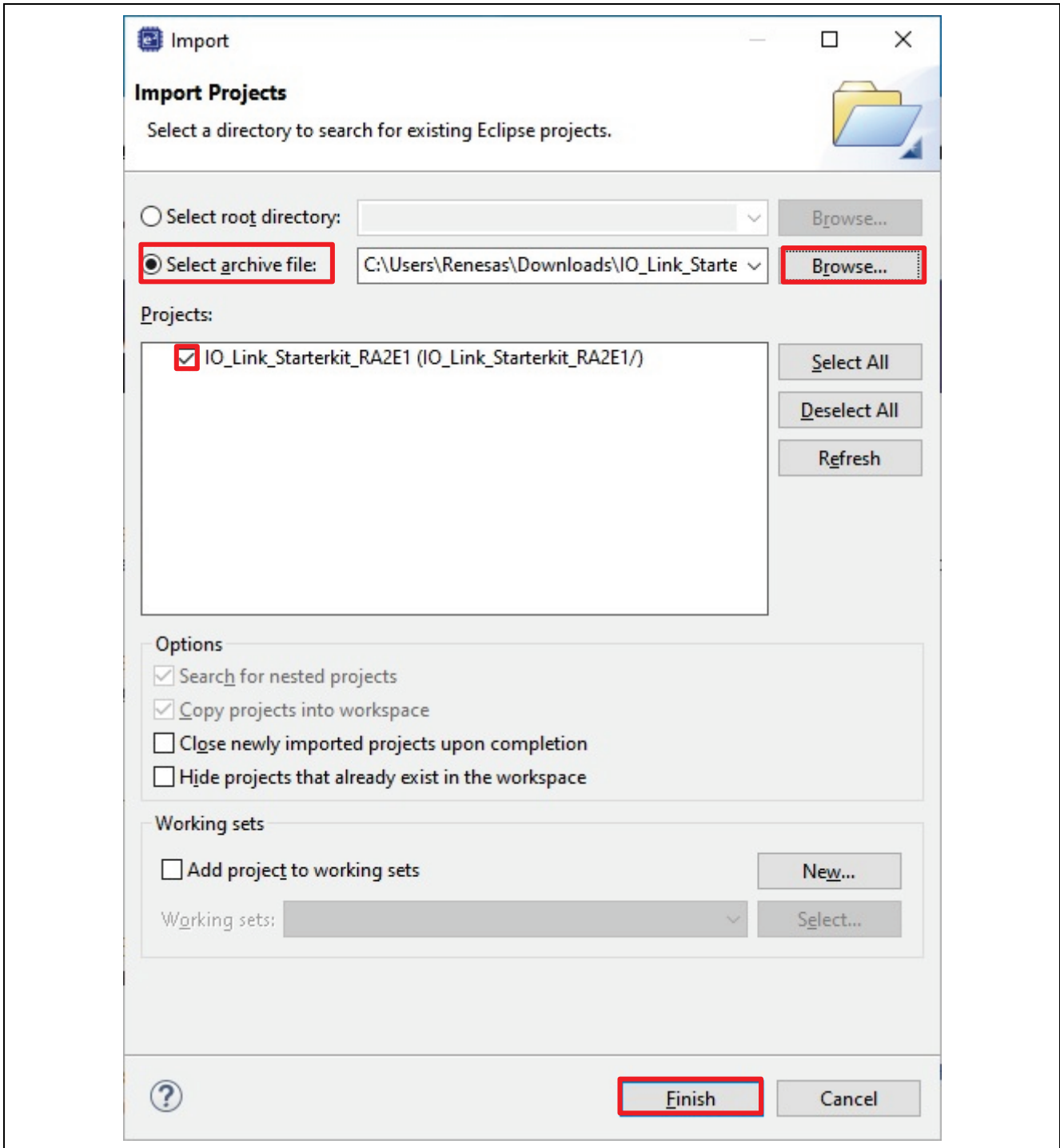
Figure 15. Importing Sample Projects
