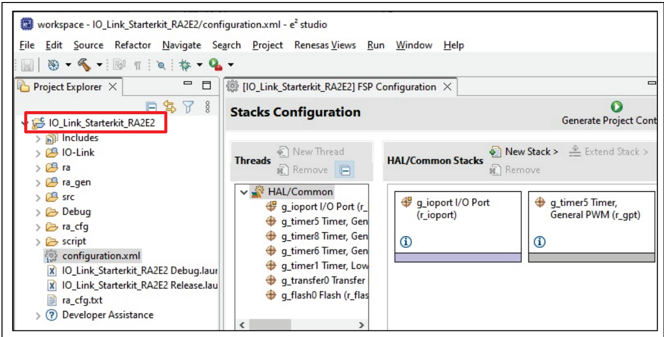
Figure 18. Build the Project
