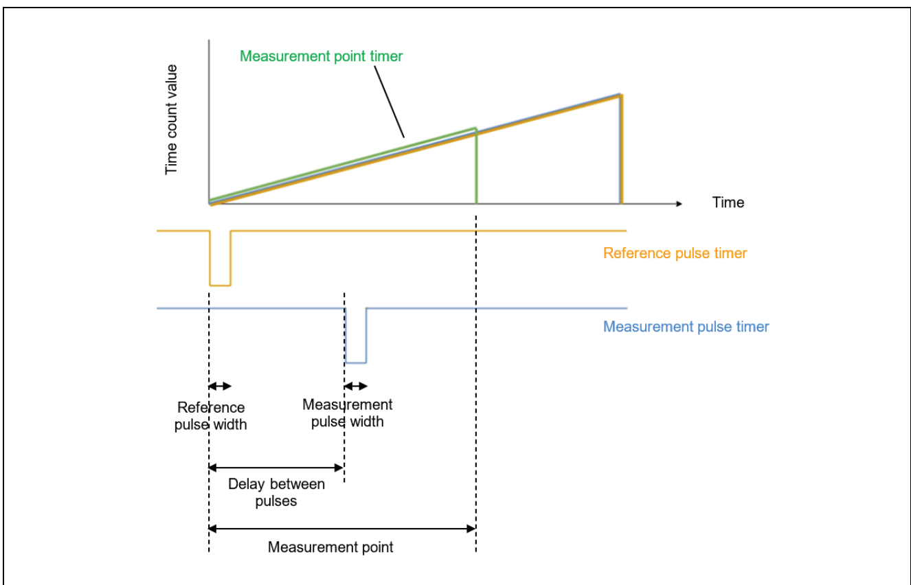
Figure 9. Pulse Generation Mechanism
