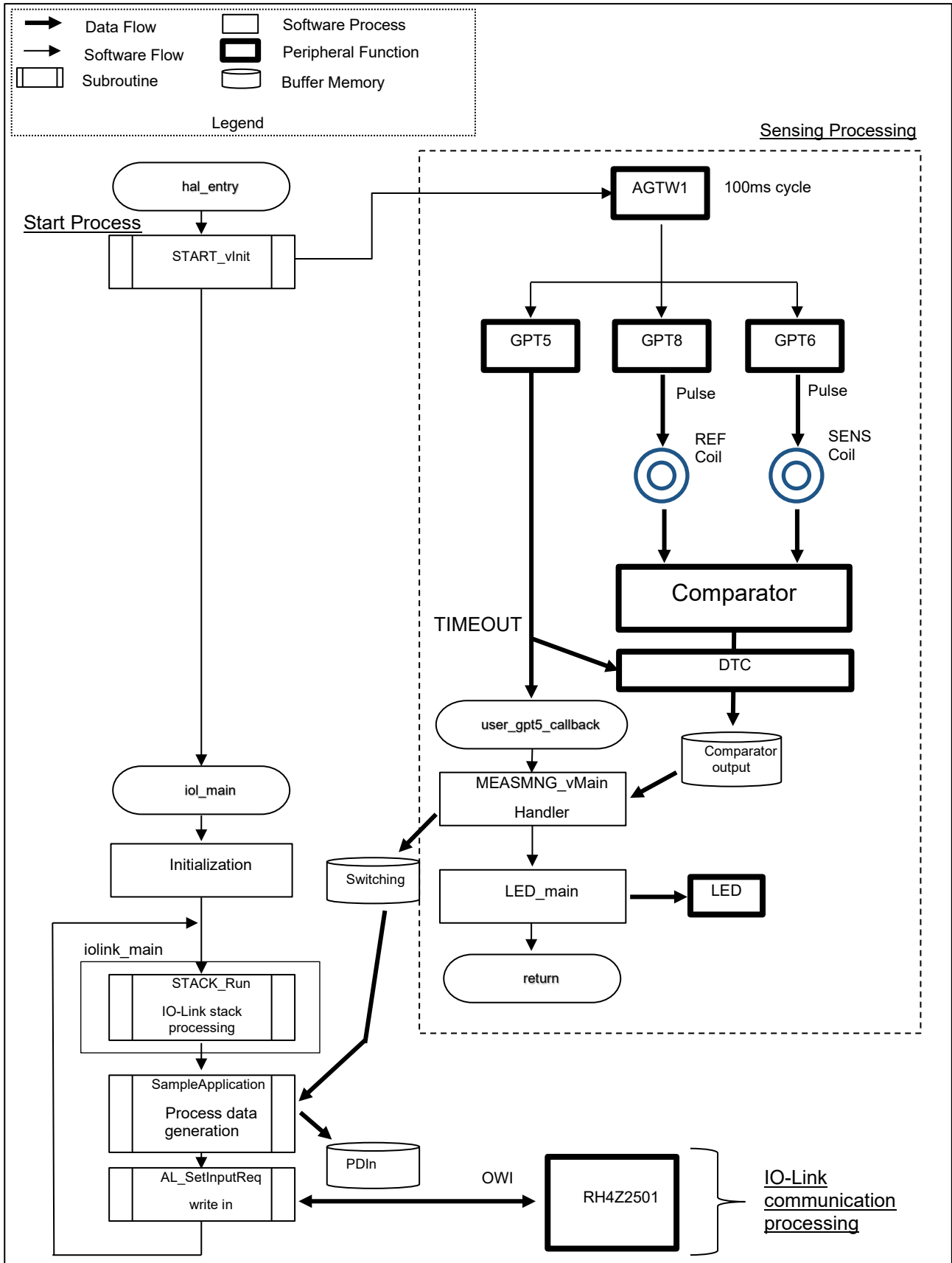
Figure 10. Processing Flow of the Sample Application
