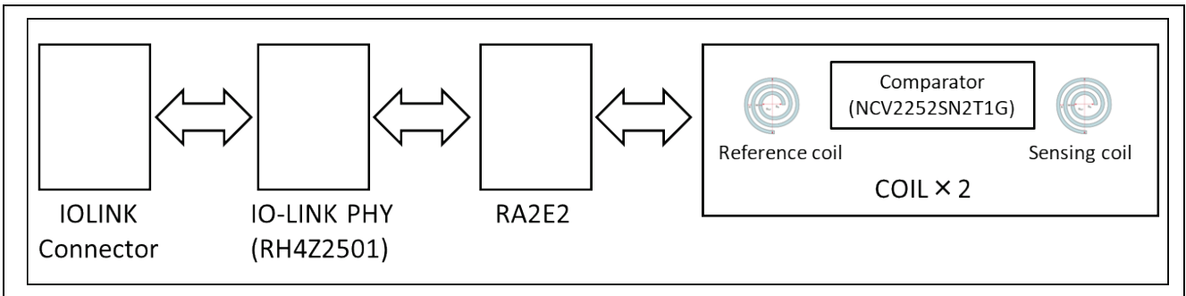
Figure 5. RA2E2 IO-Link Inductive Sensor Board Hardware Configuration
