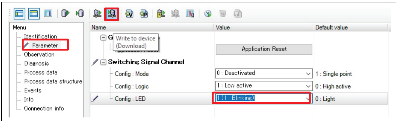
Figure 61. Config.LED Setting
