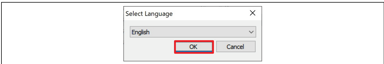
Figure 38. Select Language
