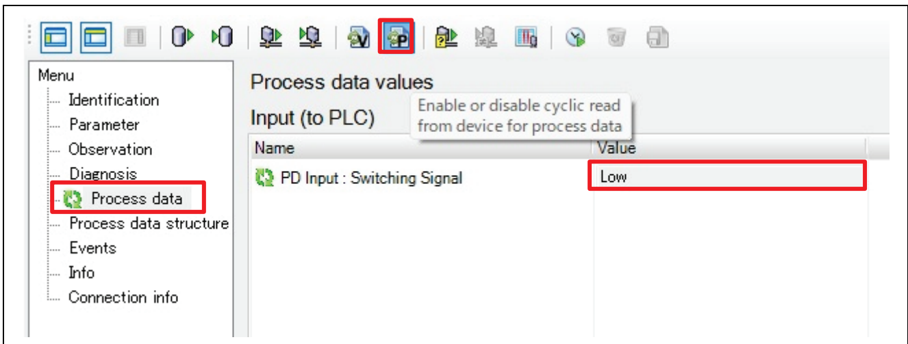
Figure 62. Process Data
