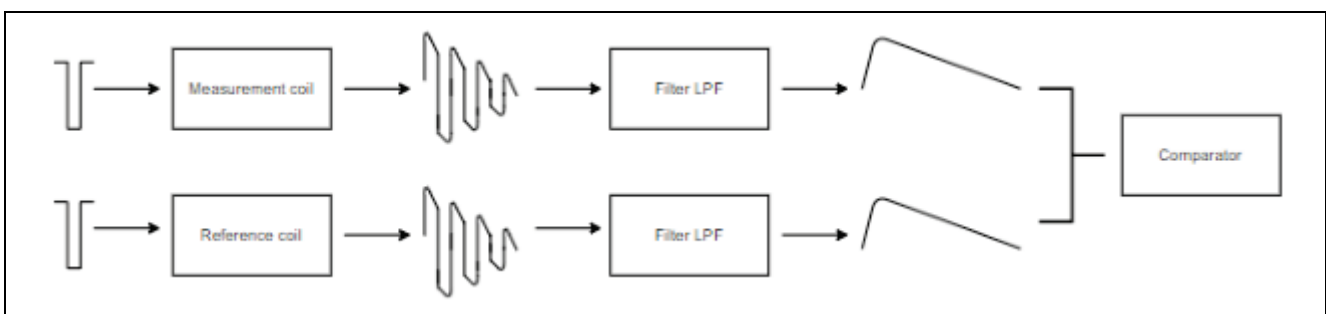
Figure 8. Operating Principle
