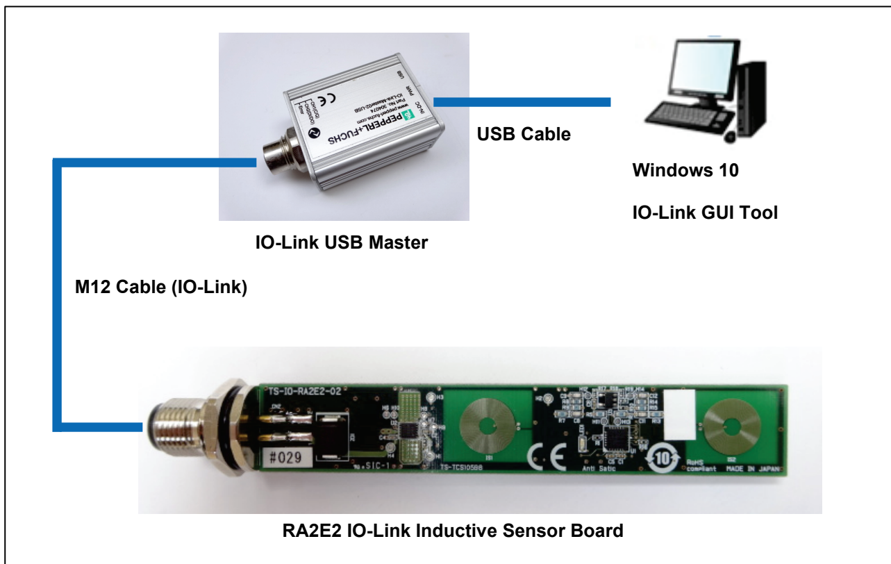
Figure 2. Hardware Configuration
