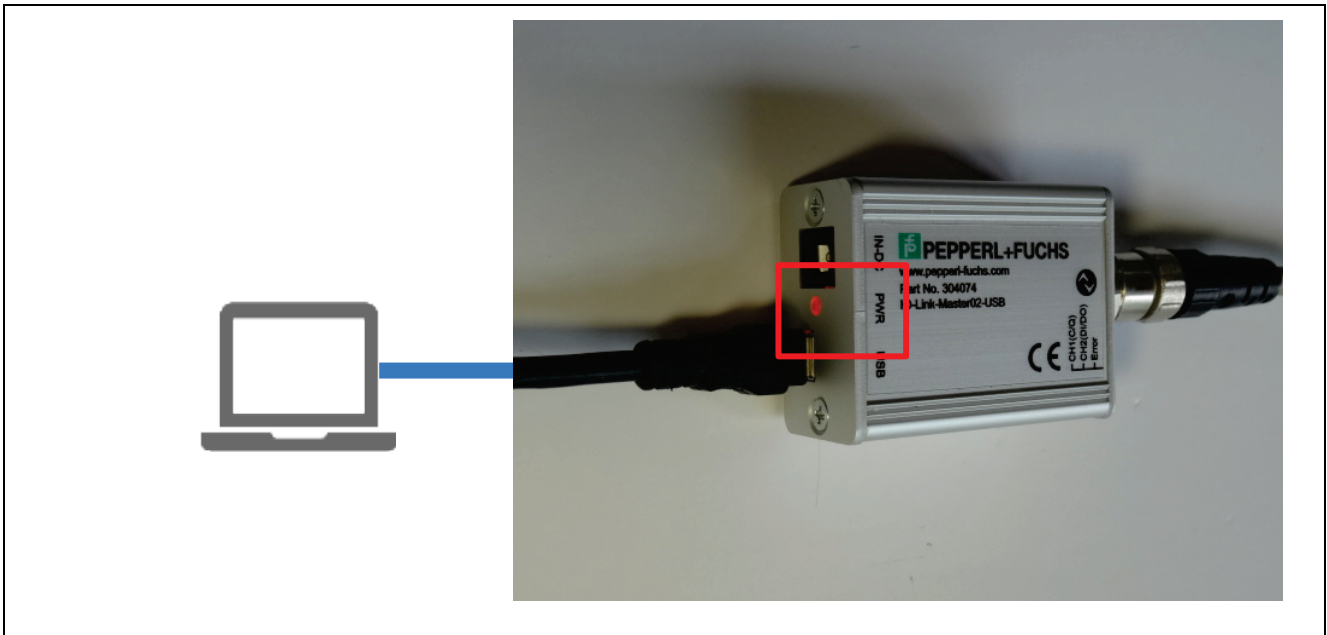
Figure 25. USB Master PC Connection
