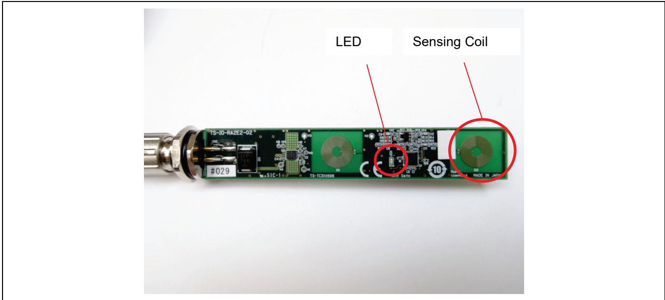
Figure 63. Metal - When Not Detected
