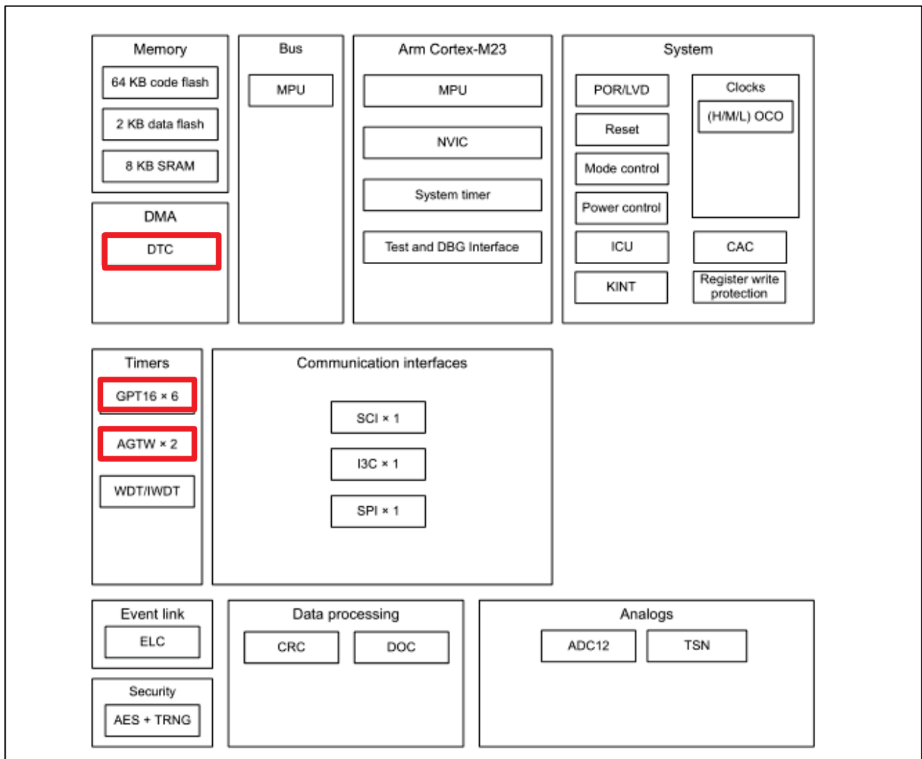
Figure 6. RA2E2 MCU Functional Overview
