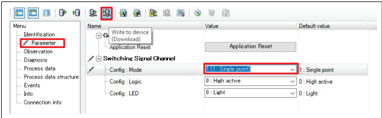
Figure 59. Config.Mode Setting
