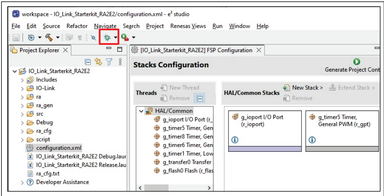
Figure 27. Launch in 'Debug' Mode
