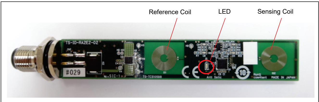
Figure 4. RA2E2 IO-Link Inductive Sensor Board
