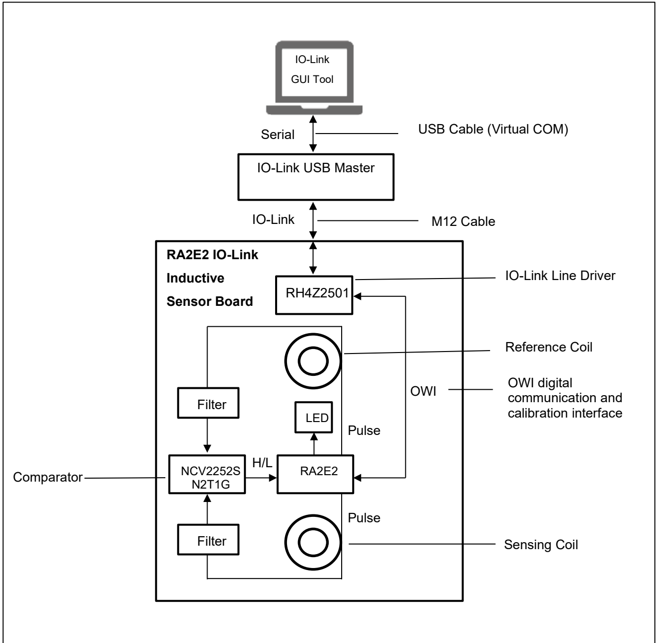
Figure 1. IO-Link Inductive Sensor System using RA2E2
