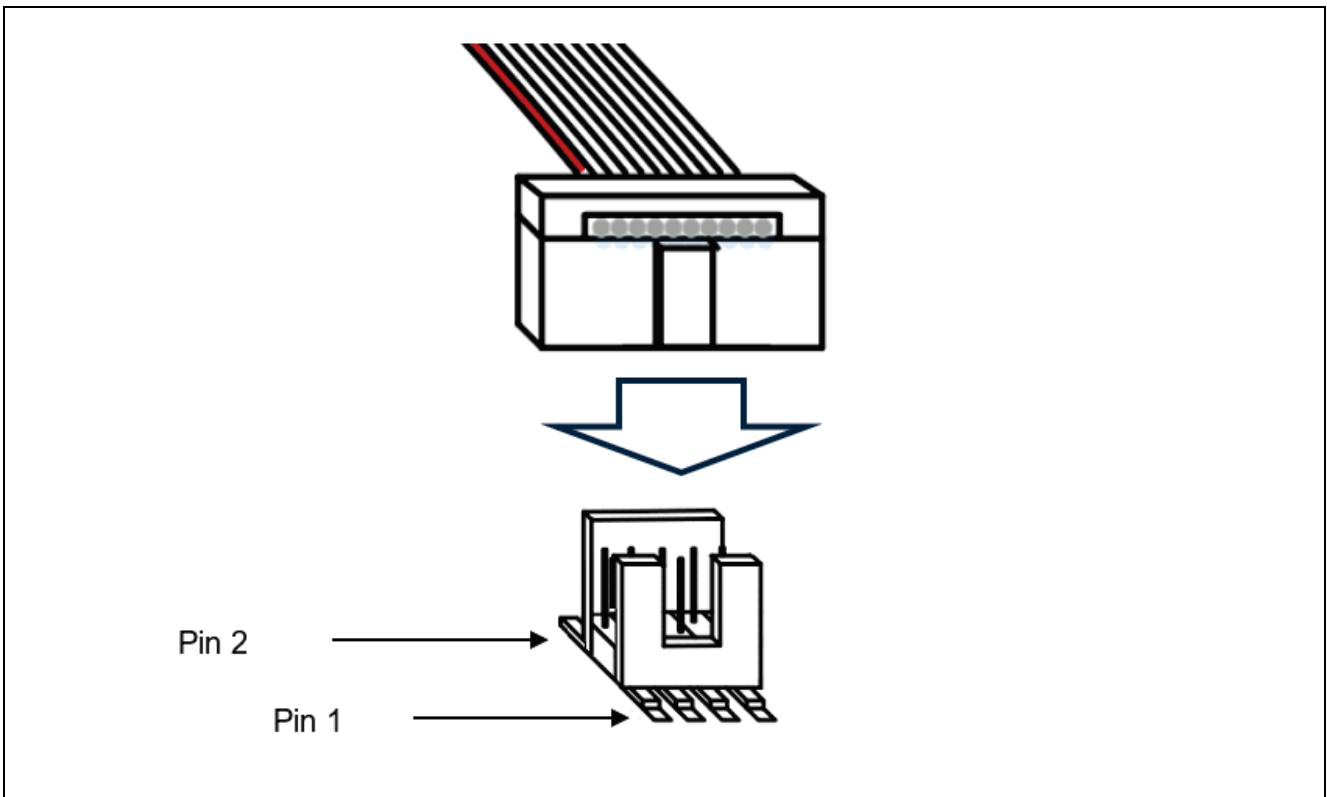
Figure 22. Connection Direction of 10-pin Connector
