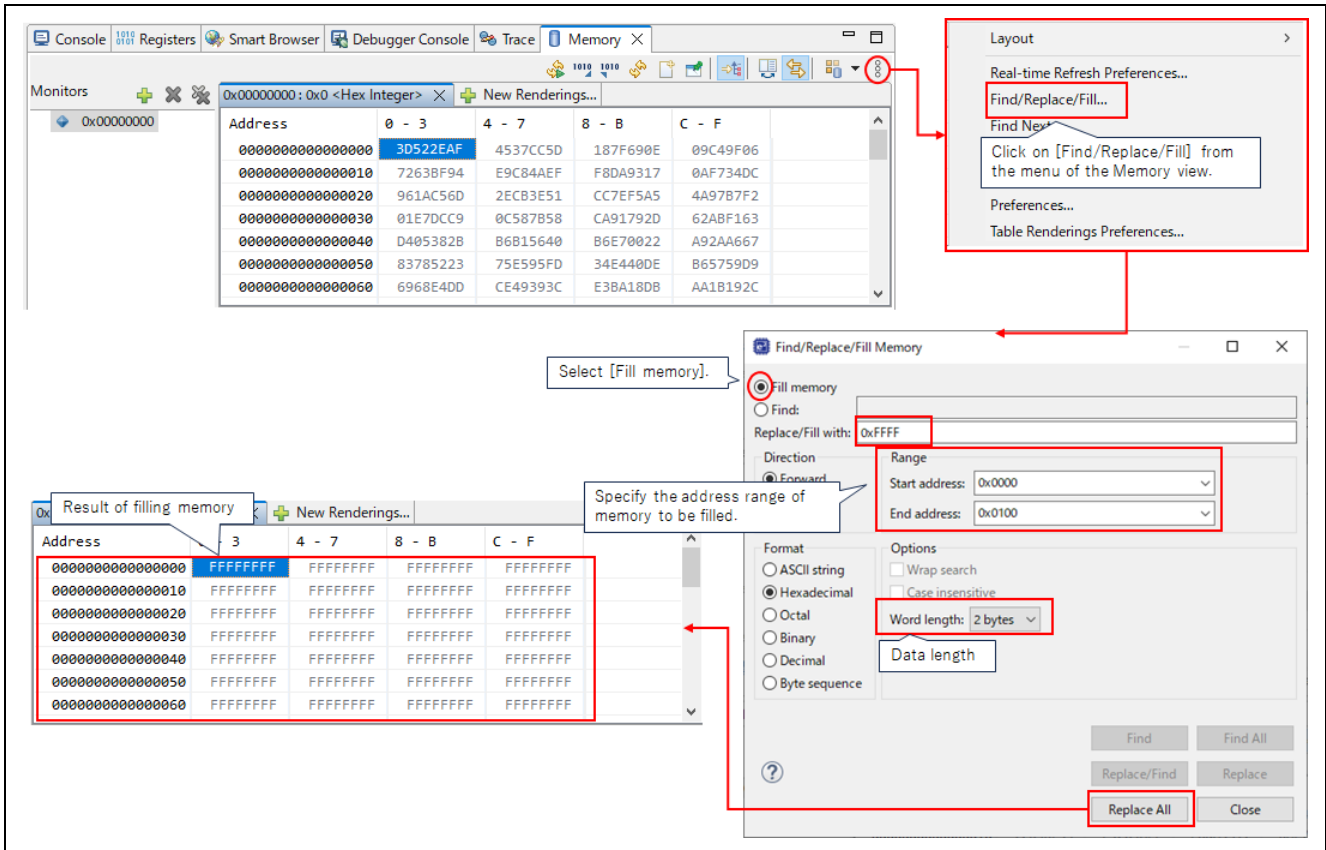
Figure 5-8 Filling Memory
