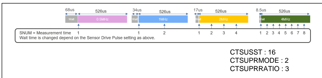
Figure 9 Self-capacitance Measurement Period (CTSU1)
