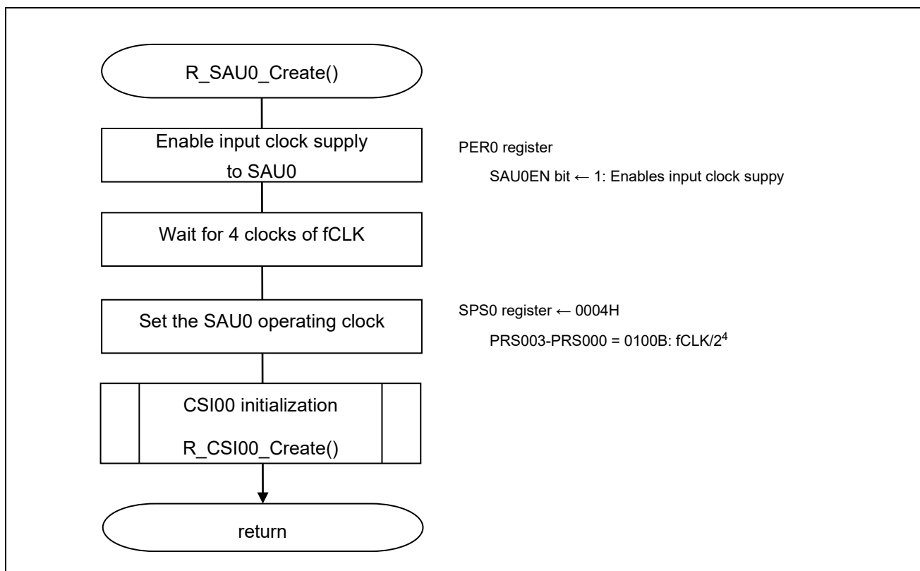
Figure 5.2 SAU0 Initialization
