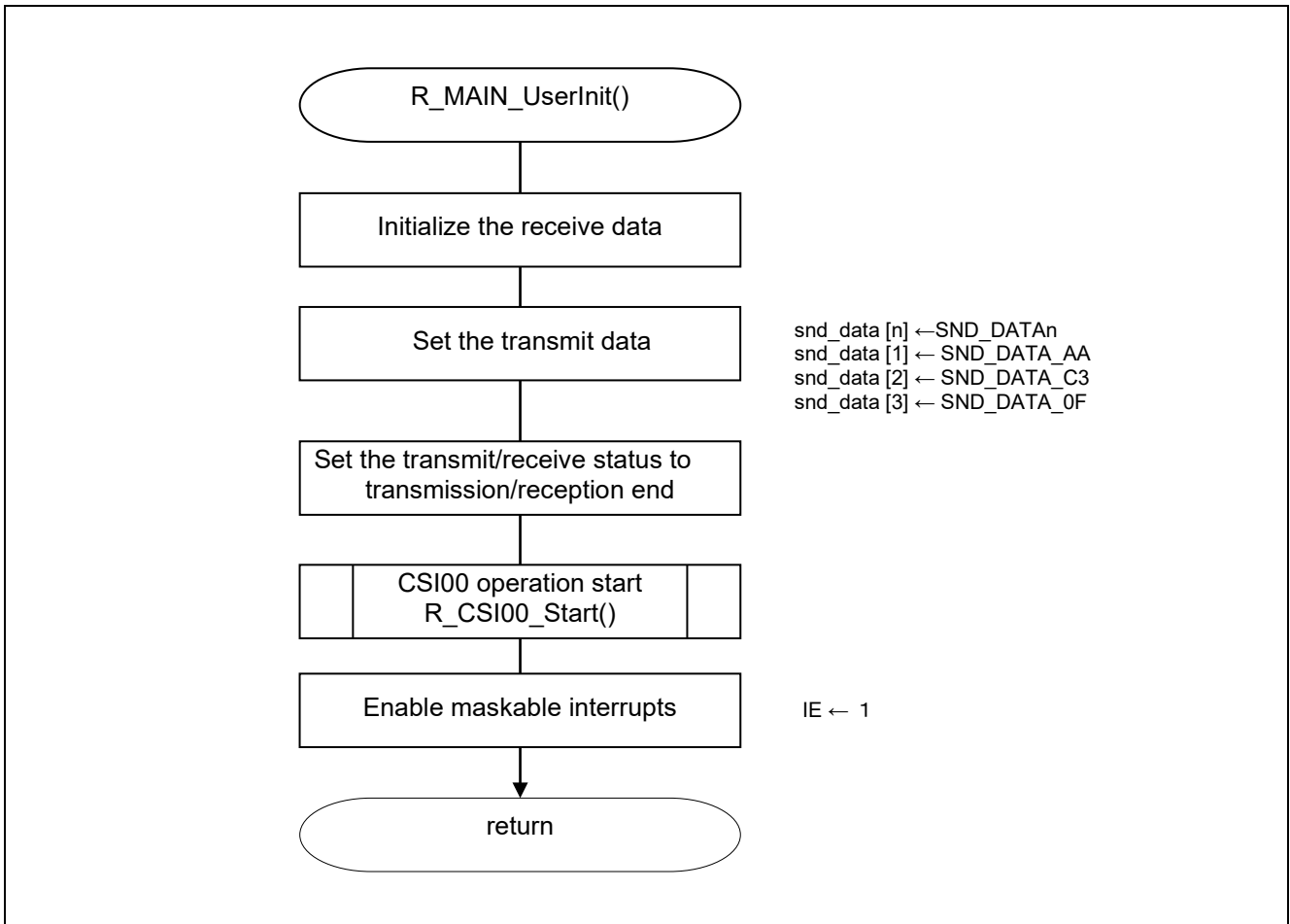
Figure 5.6 Main Initialization
