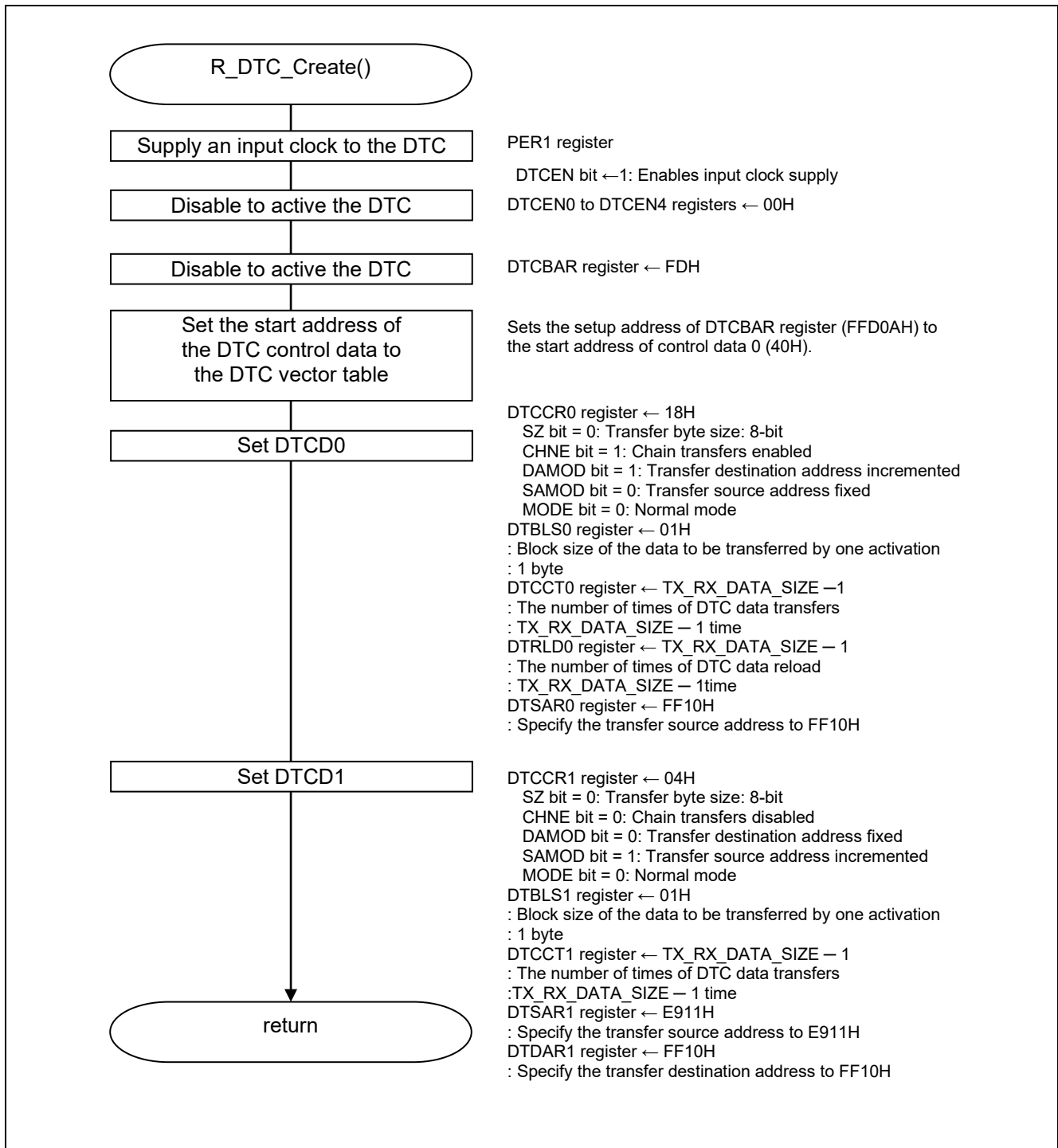
Figure 5.4 DTC Initialization
