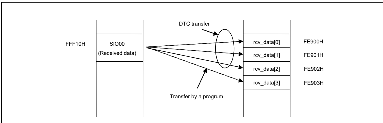
Figure 5.3 DTCD0 Operation
