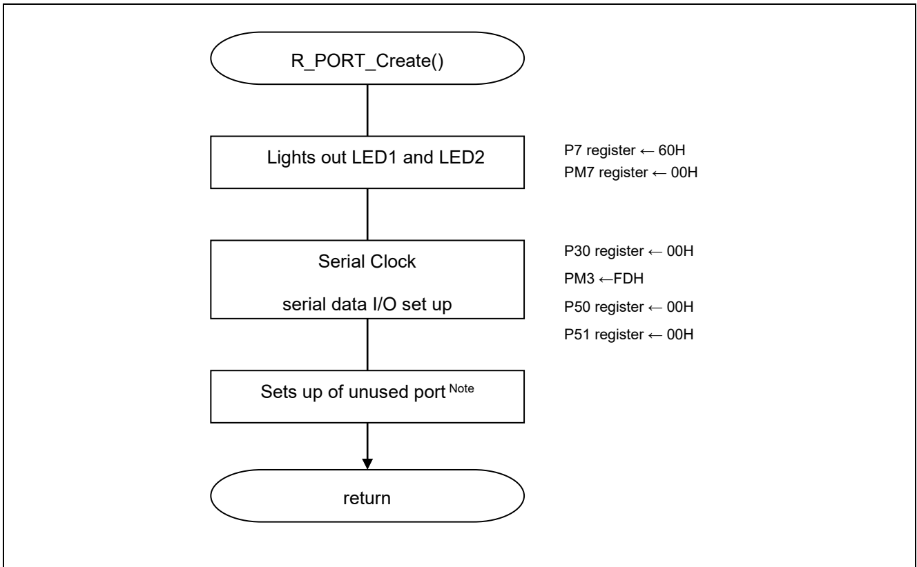
Figure 5.9 Port Initialization
