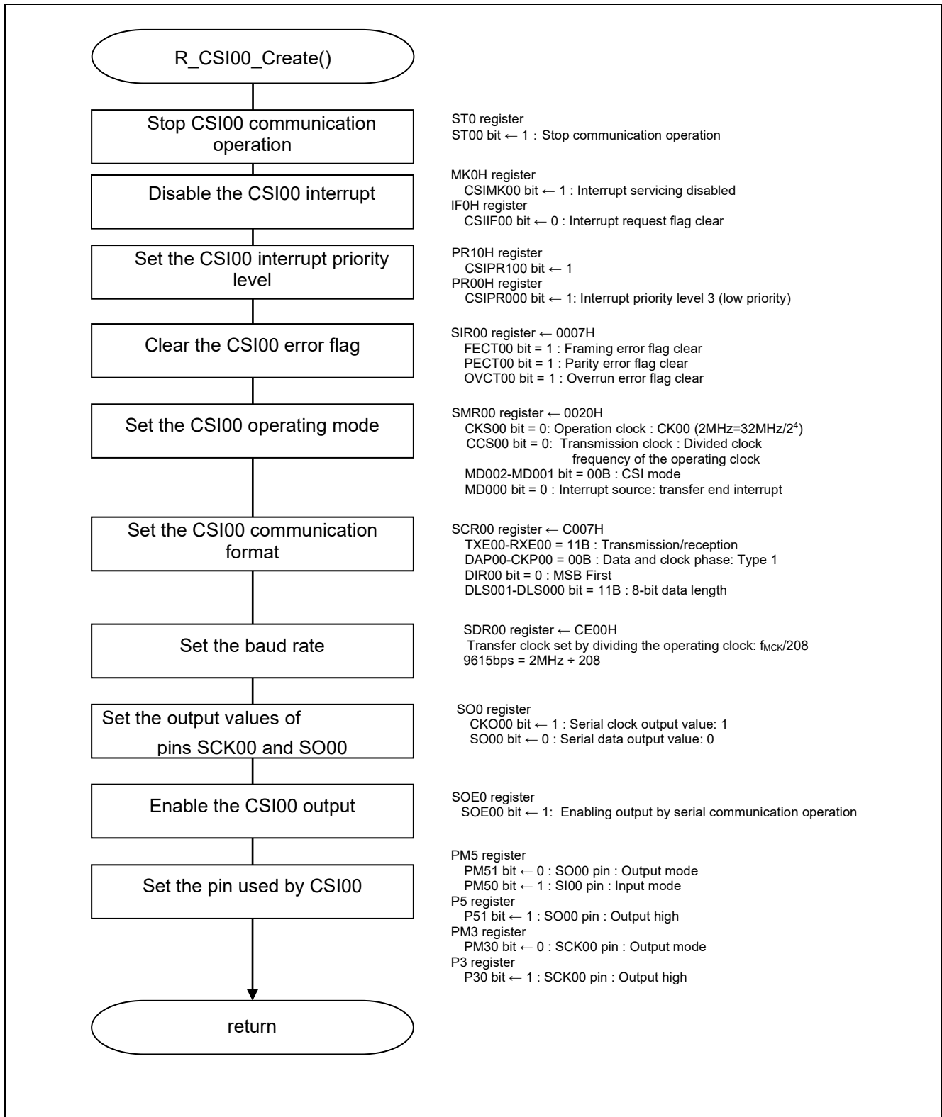
Figure 5.3 CSI00 Initialization
