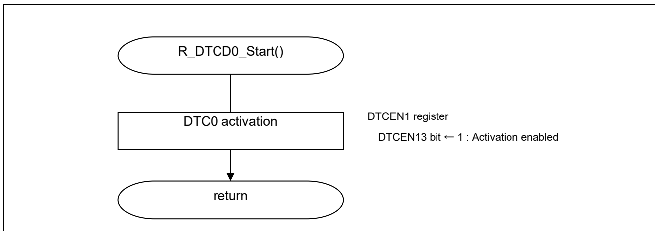
Figure 5.8 DTC0Activation
