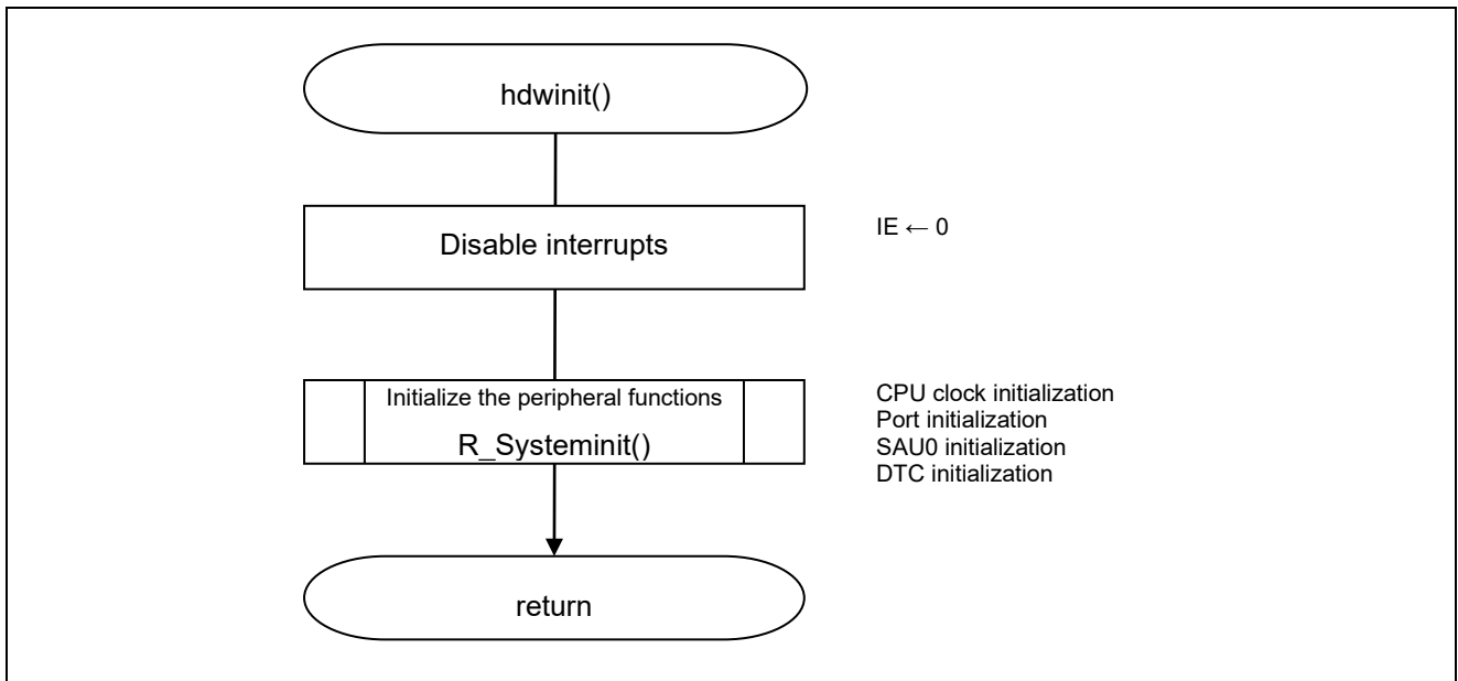
Figure 5.6 Initialization
