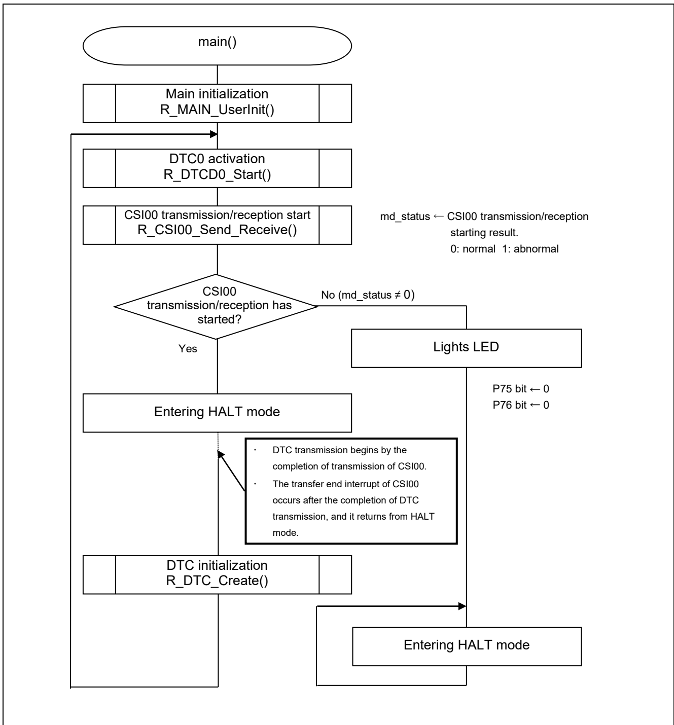
Figure 5.5 Main Processing
