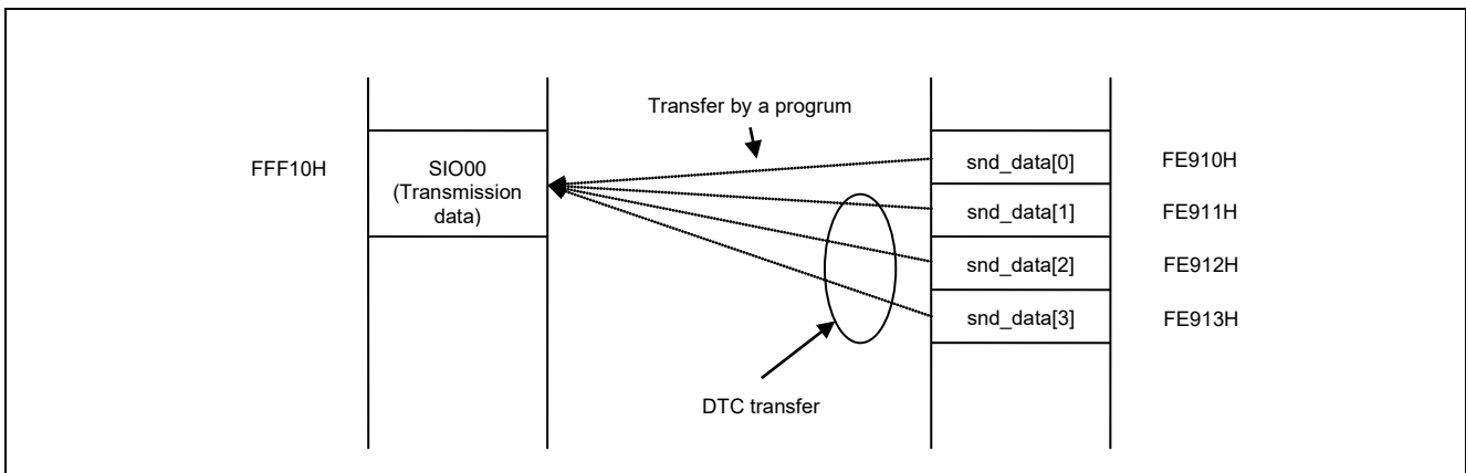
Figure 5.4 DTCD1 Operation
