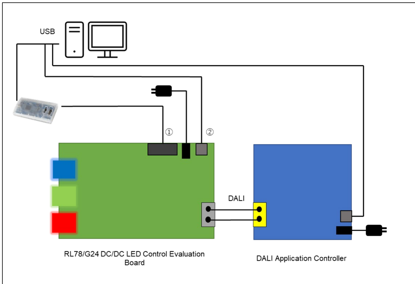
Figure 4-2 Connection diagram
